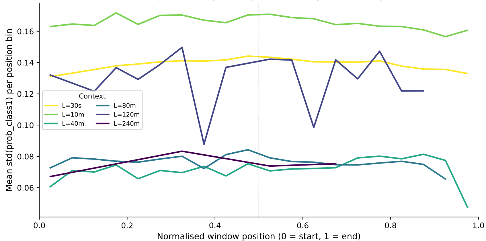
Prediction Variance vs Night Position — psqi_binary (LSTM) Lower variance = position-independent predictions (longer context may flatten this)
