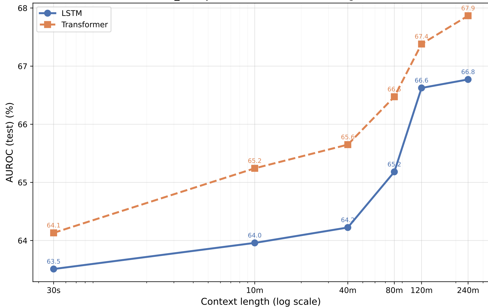
cvd_binary — AUROC vs Context Length
