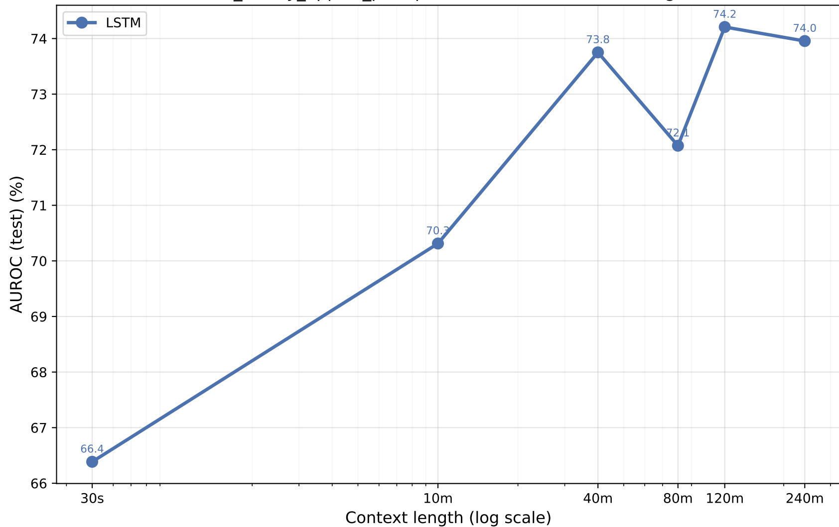
osa_binary_apples_postqc — AUROC vs Context Length
