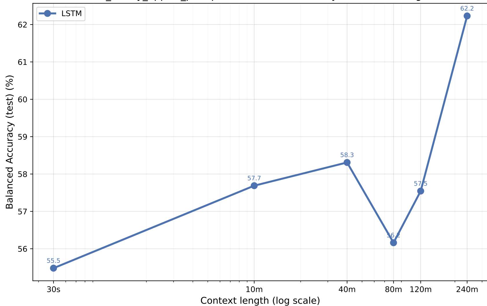
osa_binary_apples_postqc — Balanced Accuracy vs Context Length
