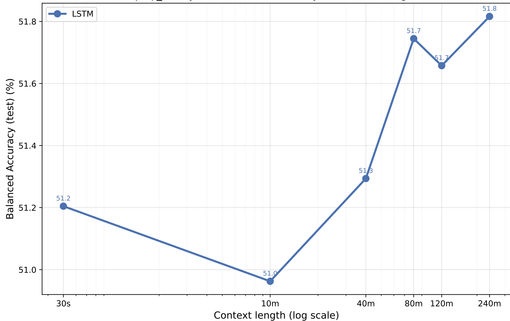
psqi_binary — Balanced Accuracy vs Context Length
