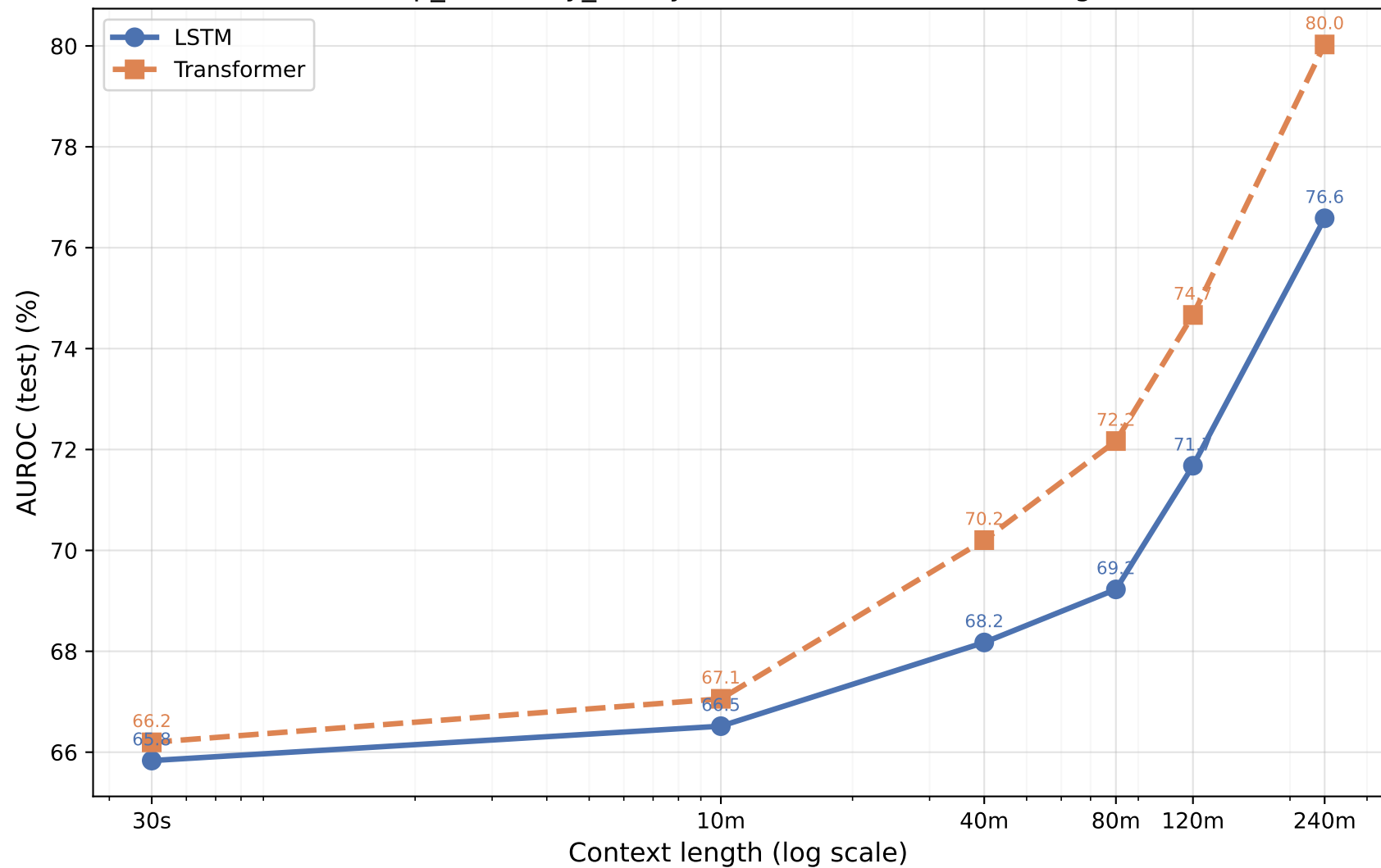
sleep_efficiency_binary — AUROC vs Context Length
