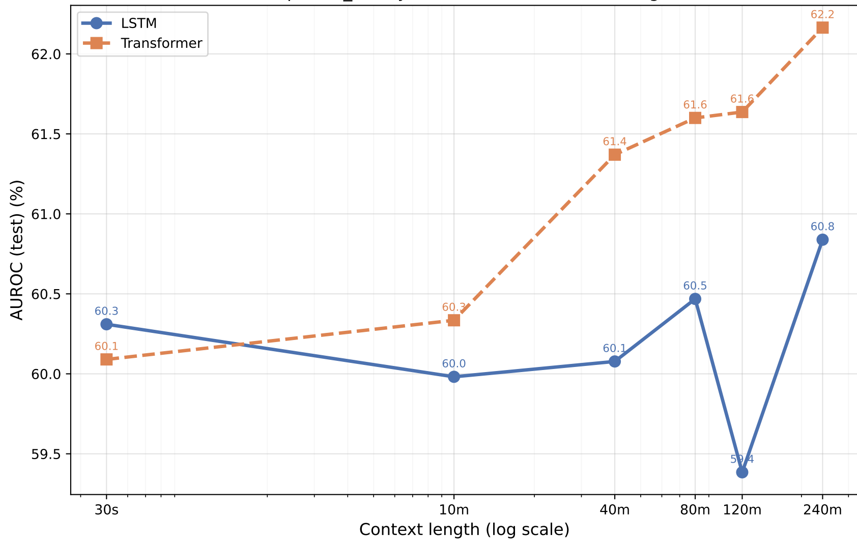
sleepiness_binary — AUROC vs Context Length
