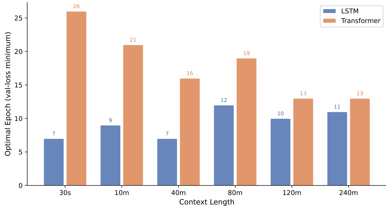
Optimal Epoch vs Context Length — apnea_binary Longer context may require more epochs to converge
