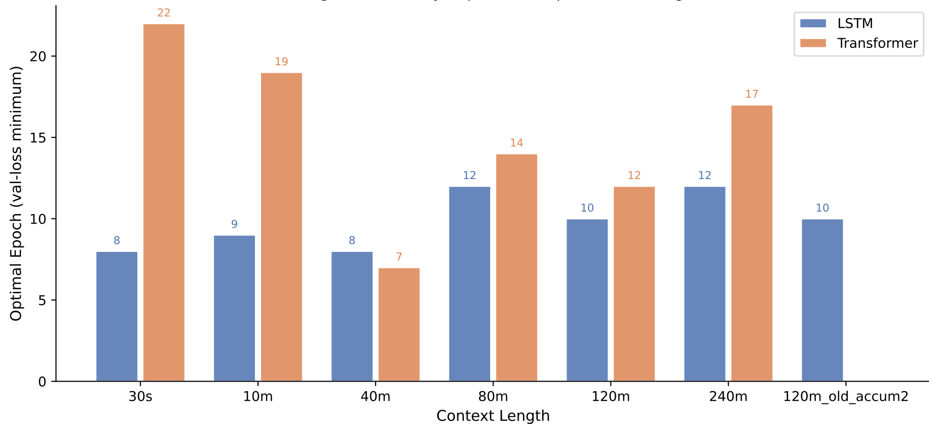
Optimal Epoch vs Context Length — bmi_binary Longer context may require more epochs to converge
