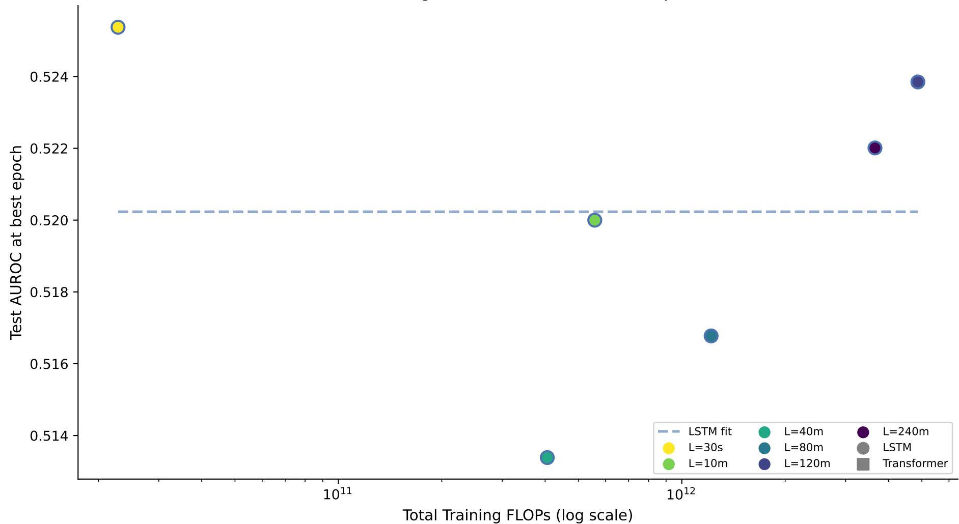
Compute Scaling Law — psqi_binary Color = context length · Marker = head · Dashed = power-law fit
