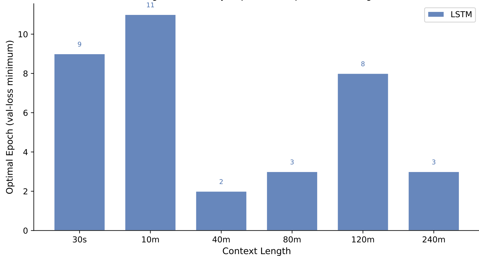
Optimal Epoch vs Context Length — psqi_binary Longer context may require more epochs to converge
