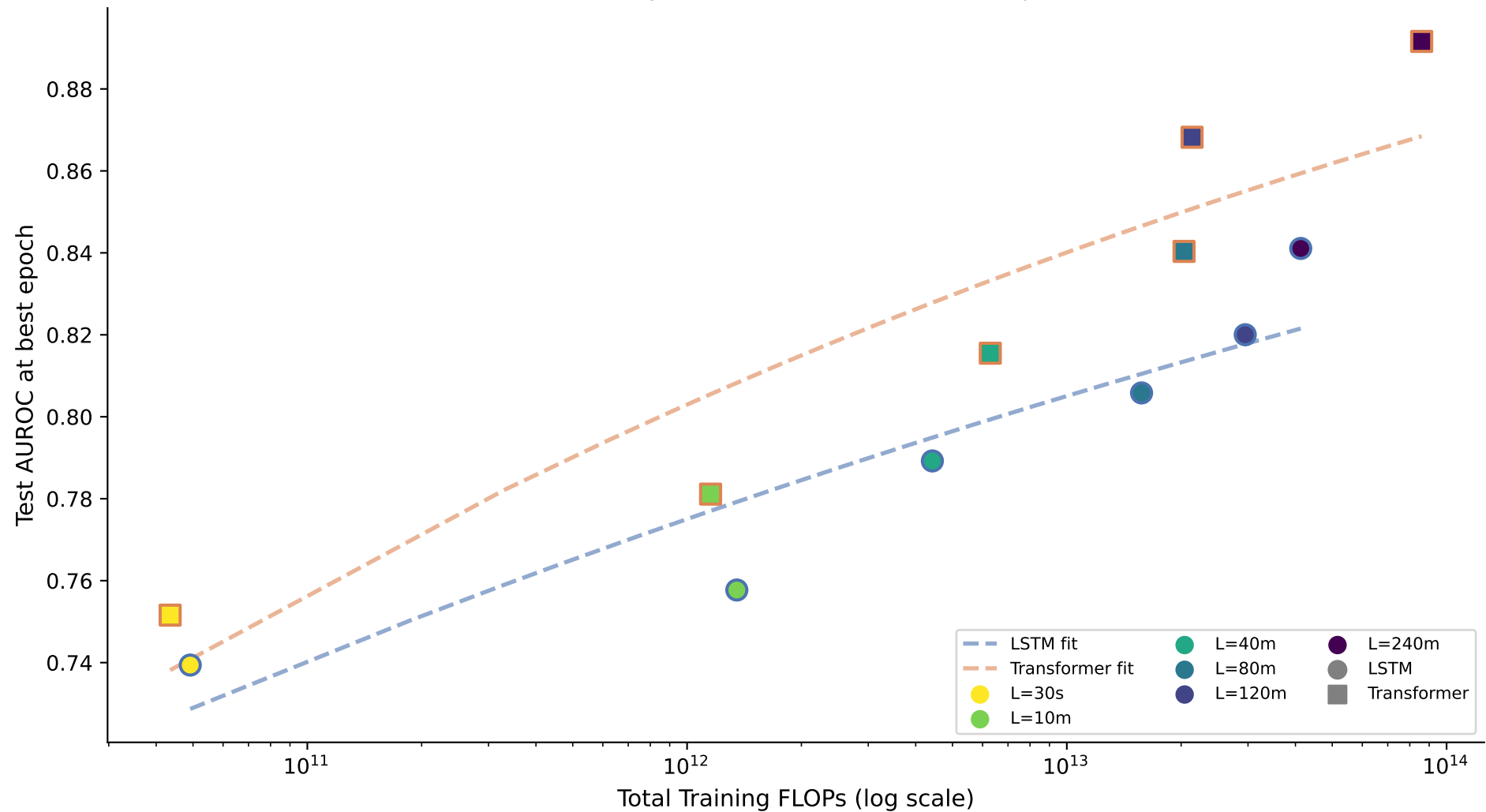
Compute Scaling Law — sex_binary Color = context length · Marker = head · Dashed = power-law fit
