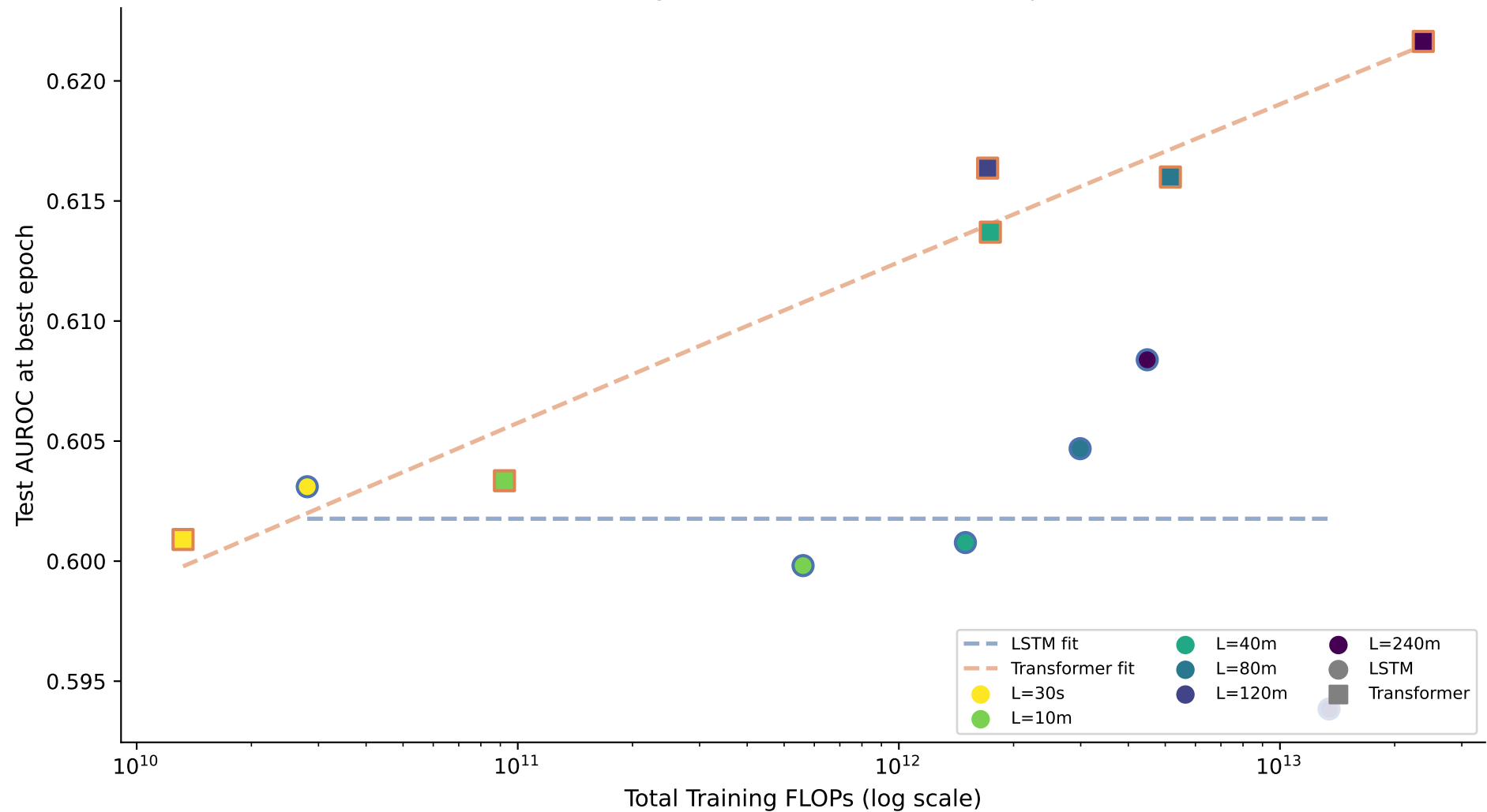
Compute Scaling Law — sleepiness_binary Color = context length · Marker = head · Dashed = power-law fit
