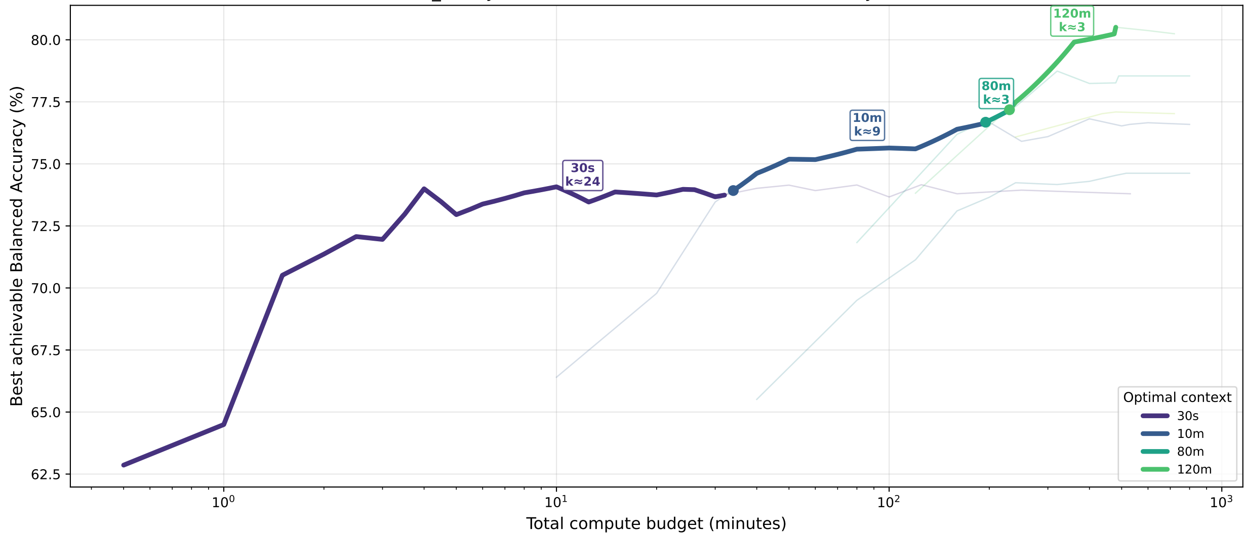
sex_binary · Istm — Pareto Front: Balanced Accuracy (%)
