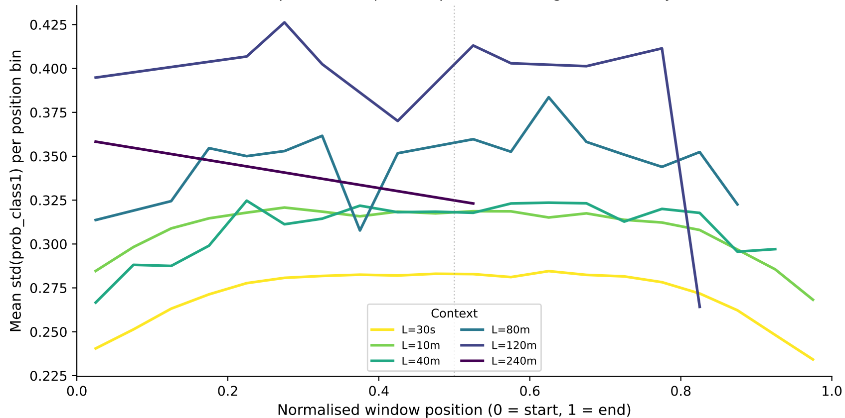
Prediction Variance vs Night Position — sex_binary (LSTM) Lower variance = position-independent predictions (longer context may flatten this)
