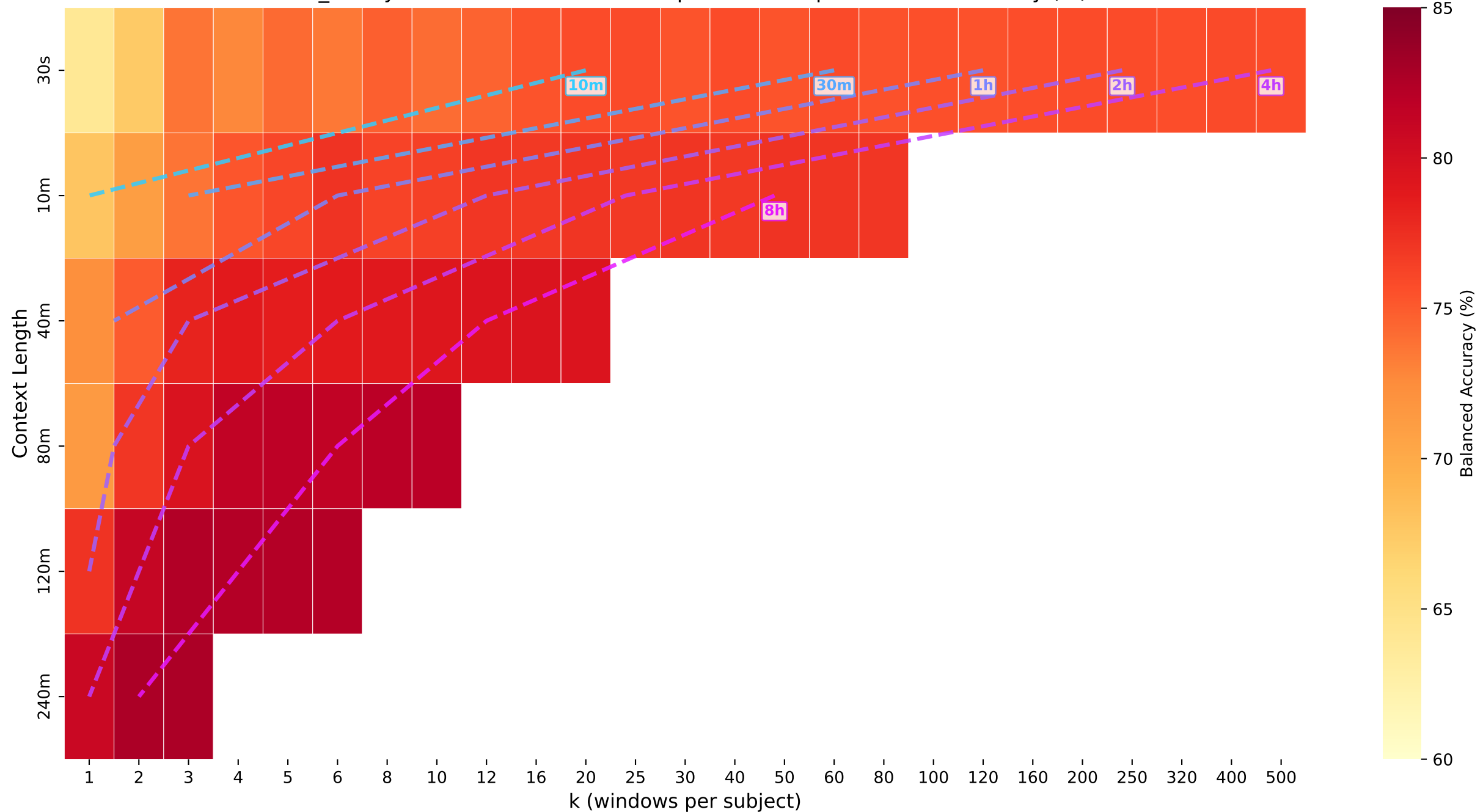
sex_binary · transformer — Iso-Compute Heatmap: Balanced Accuracy (%)
