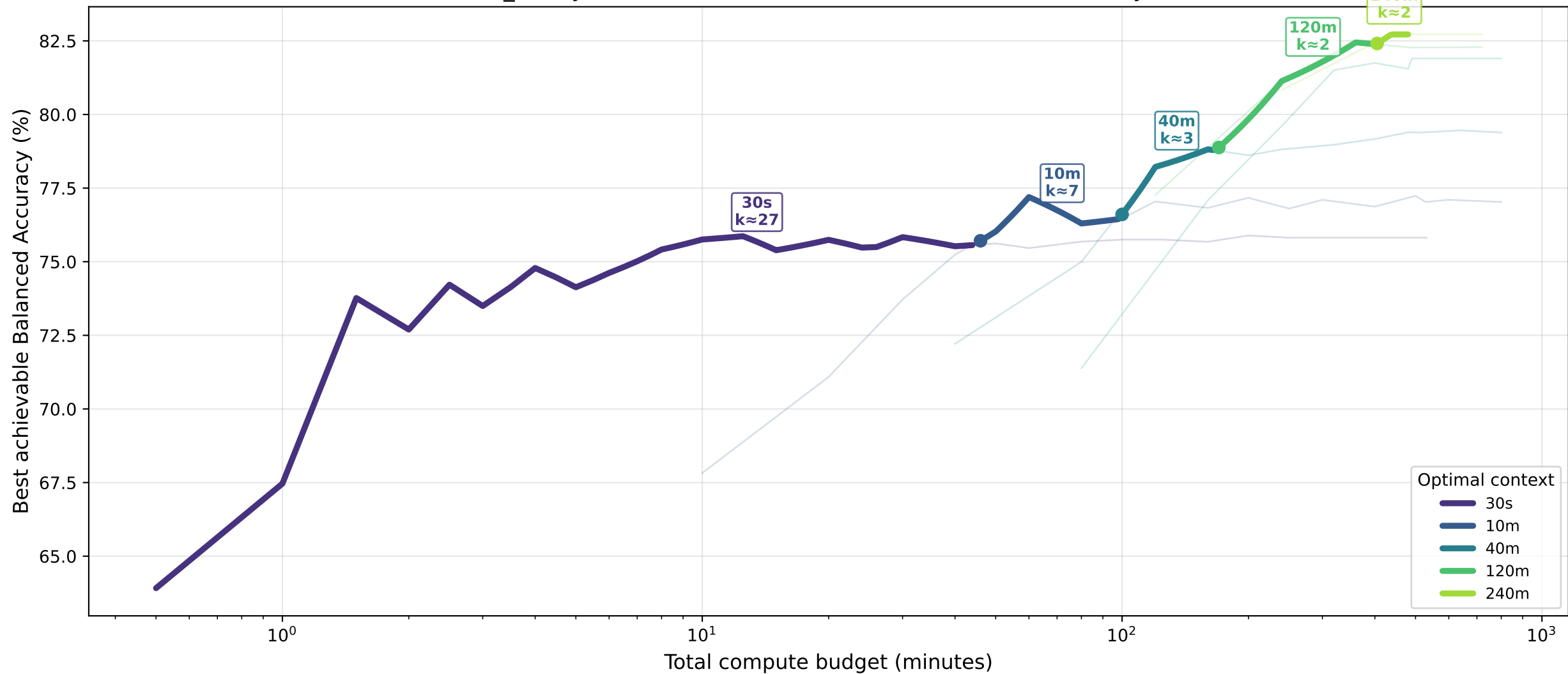
sex_binary · transformer — Pareto Front: Balanced Accuracy (%)
