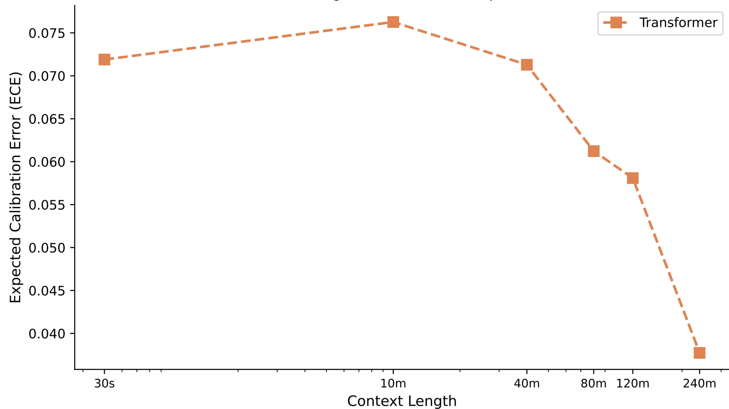
ECE vs Context Length — sex_binary (K=10) Lower is better; longer context should improve calibration
