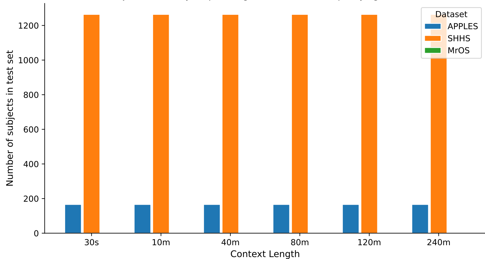
Test-Set Subject Count per Dataset — sex_binary (TRANSFORMER) Subject count may drop at longer contexts (fewer qualifying windows)
