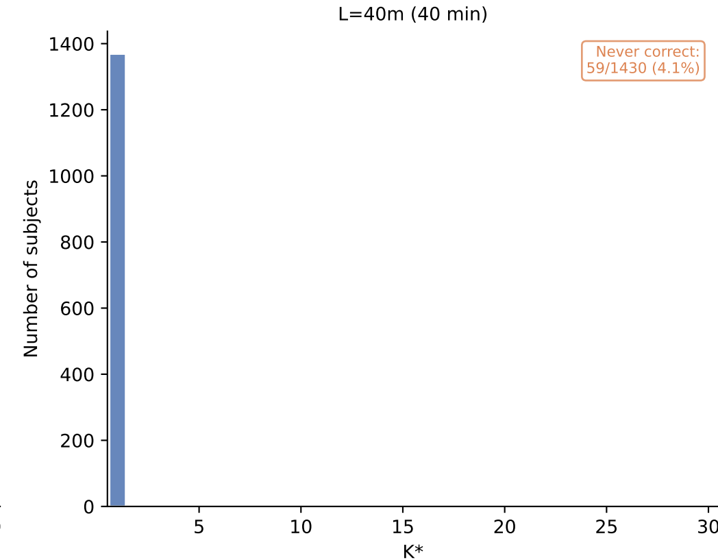
K* Distribution — sex_binary (TRANSFORMER) K* = minimum windows for correct classification (reps=20)
