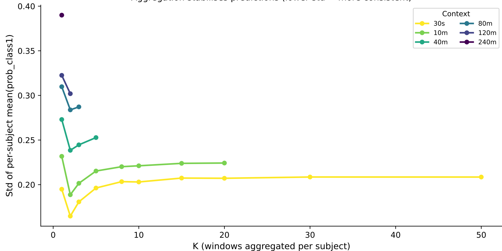
Prediction Variance vs K — sex_binary (TRANSFORMER) Aggregation stabilises predictions (lower std = more consistent)
