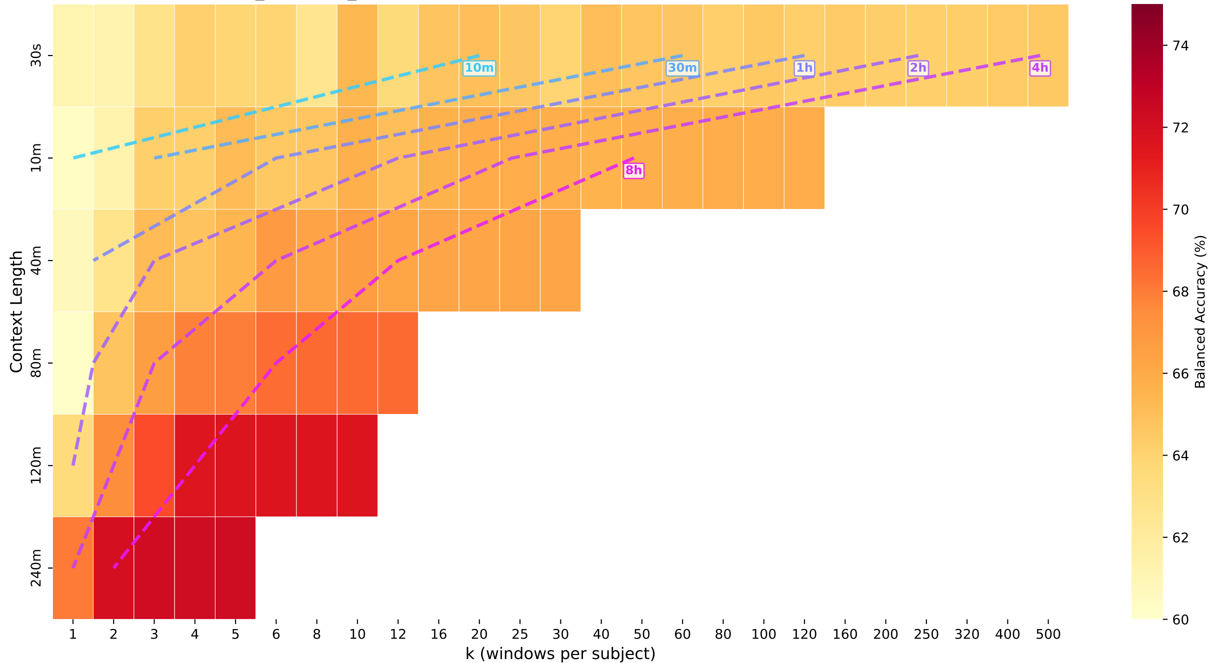
sleep_efficiency_binary · lstm — Iso-Compute Heatmap: Balanced Accuracy (%)
