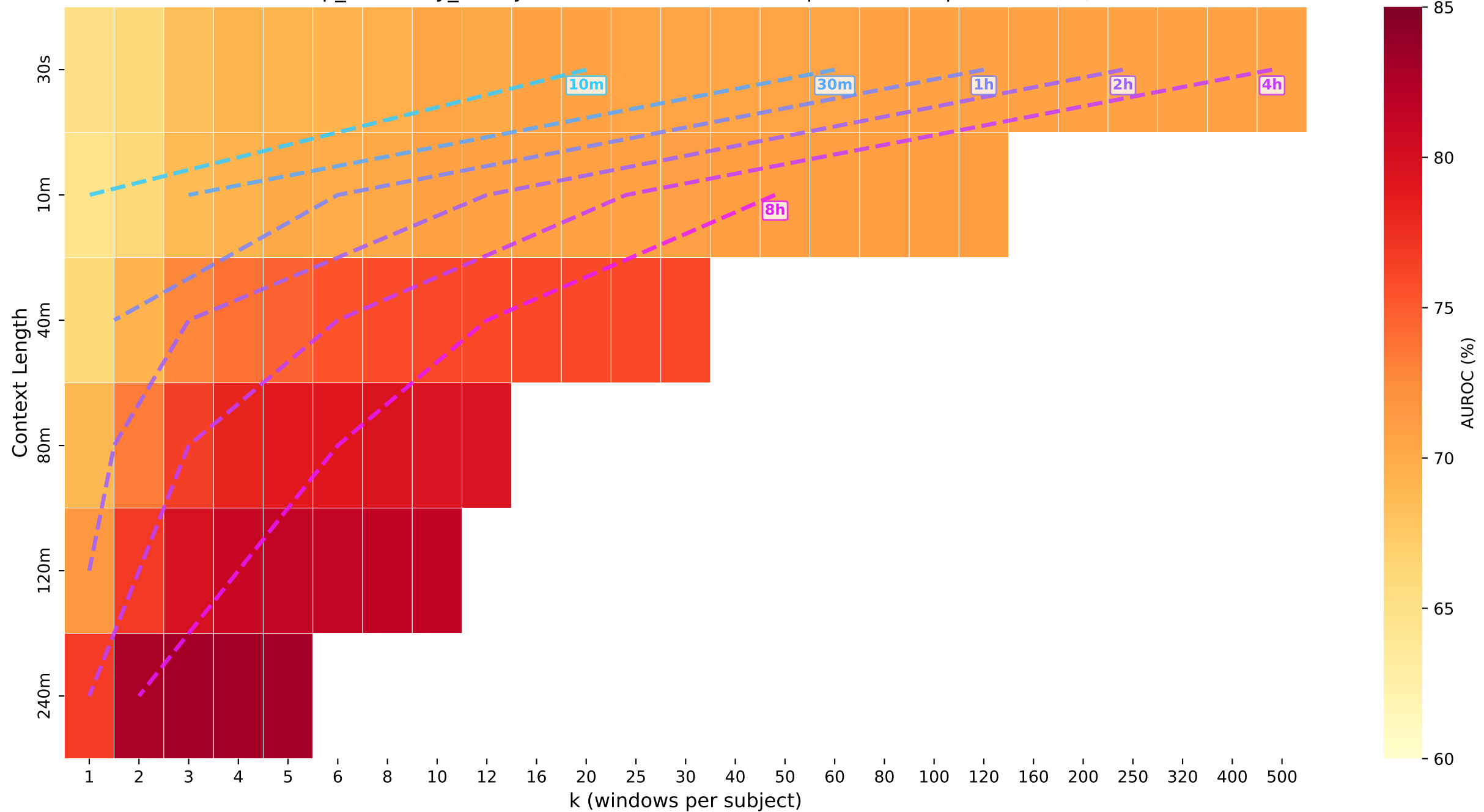
sleep_efficiency_binary · transformer — Iso-Compute Heatmap: AUROC (%)
