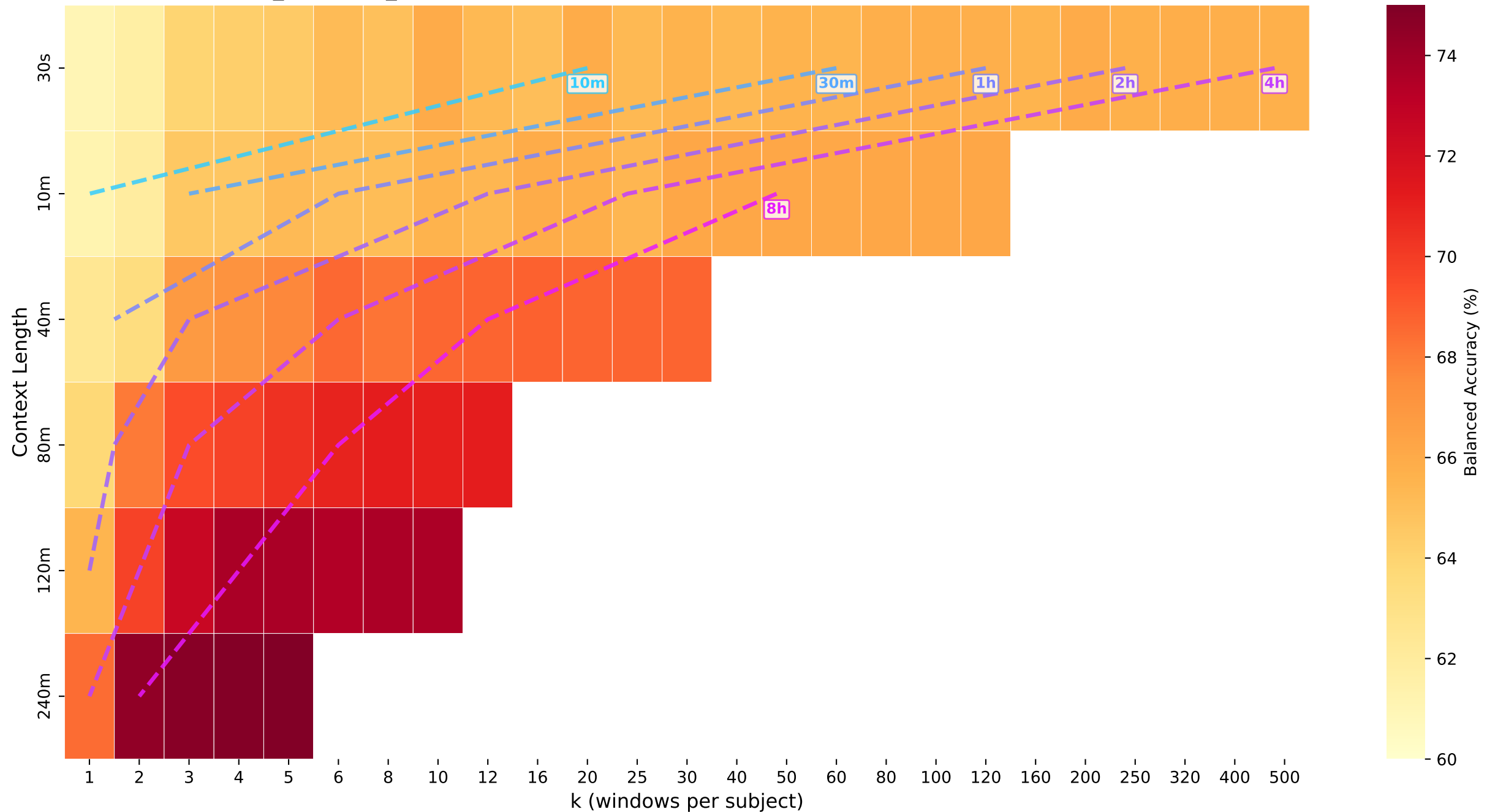
sleep_efficiency_binary · transformer — Iso-Compute Heatmap: Balanced Accuracy (%)
