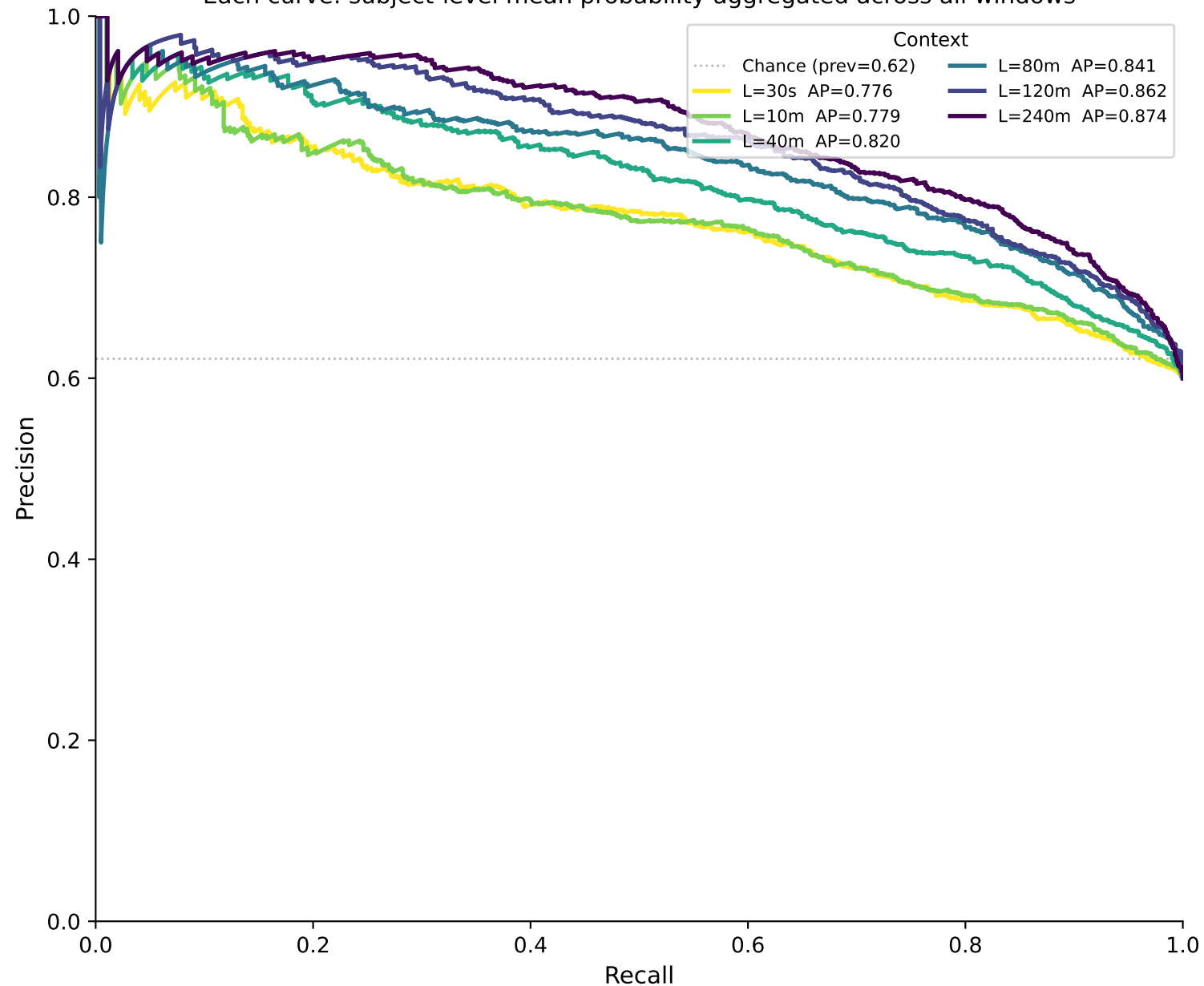
Precision-Recall Curves — sleep_efficiency_binary (TRANSFORMER) K=all Each curve: subject-level mean probability aggregated across all windows
