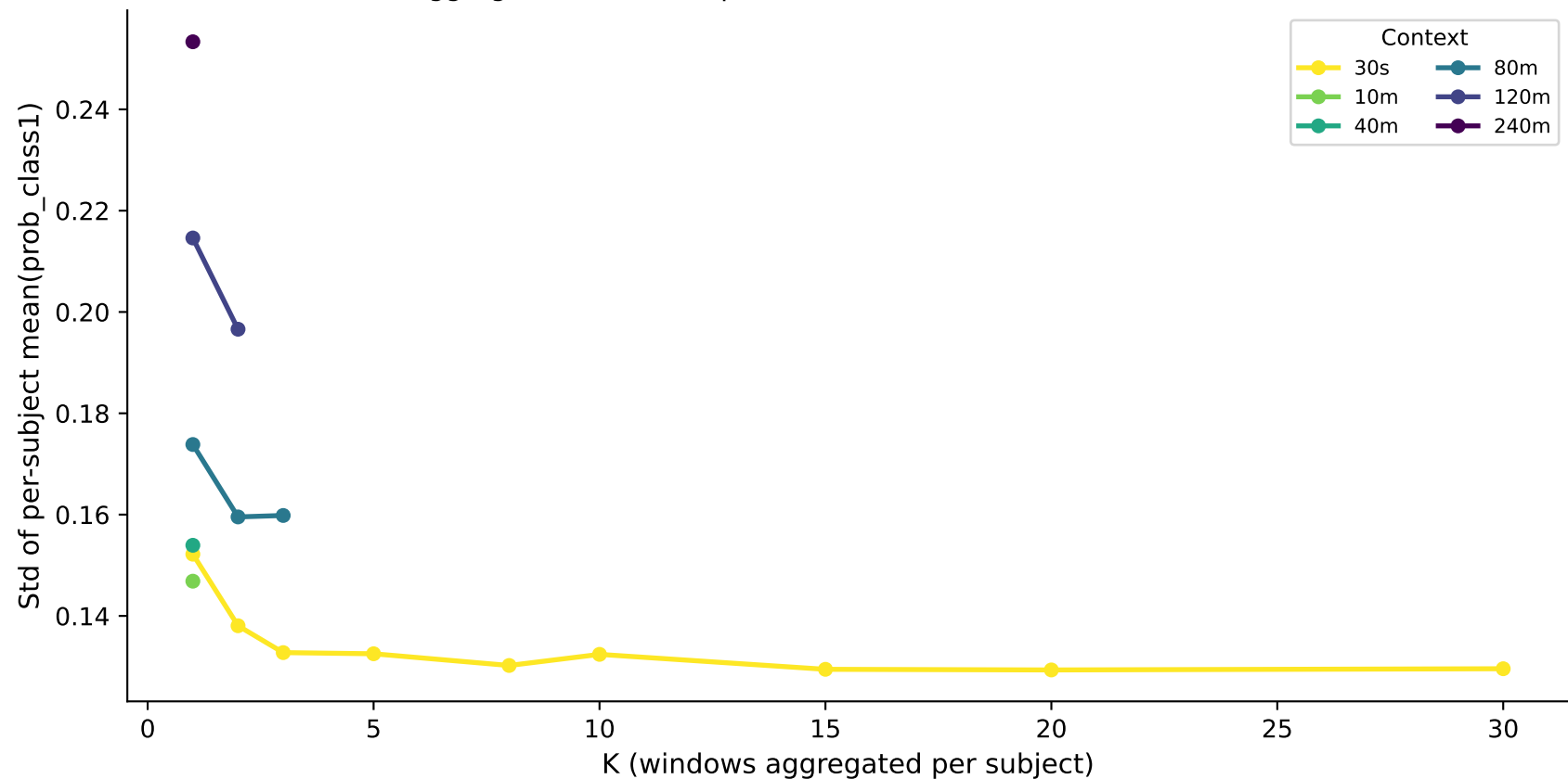
Prediction Variance vs K — sleep_efficiency_binary (TRANSFORMER) Aggregation stabilises predictions (lower std = more consistent)
