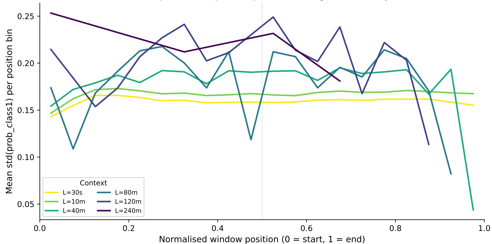
Prediction Variance vs Night Position — sleep_efficiency_binary (TRANSFORMER) Lower variance = position-independent predictions (longer context may flatten this)
