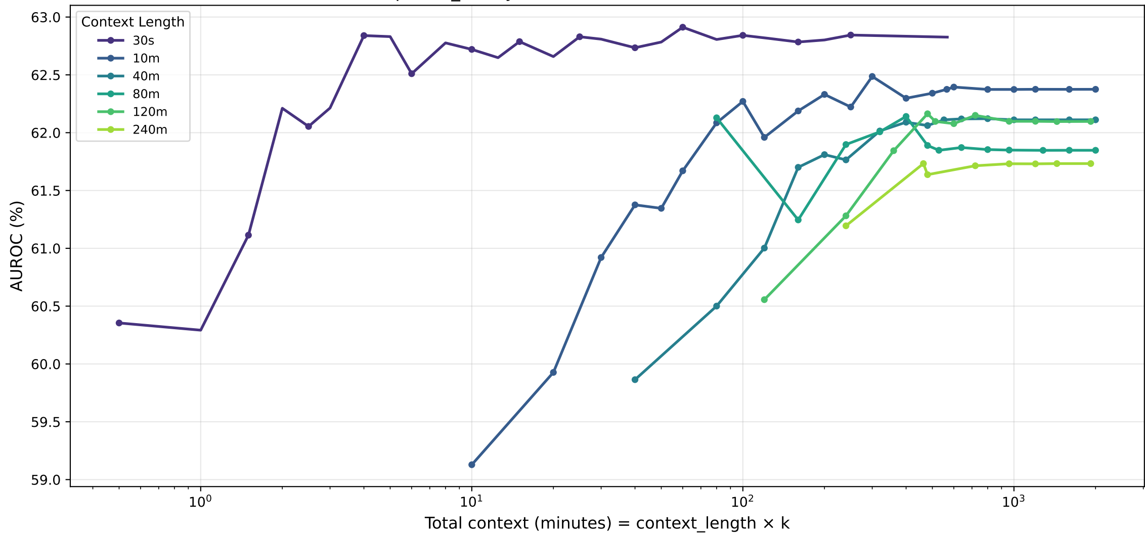
sleepiness_binary · lstm — AUROC (%) vs Total Context
