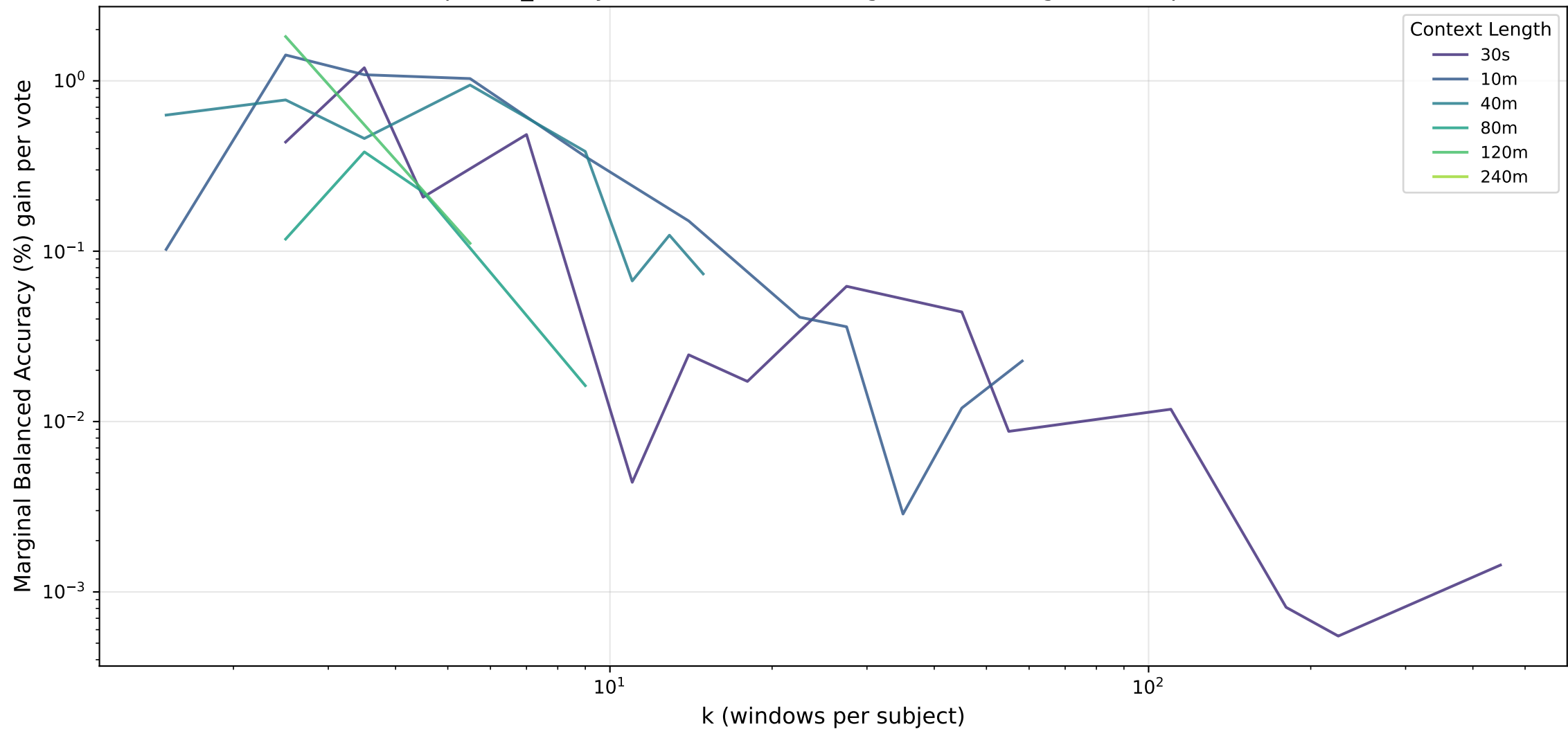
sleepiness_binary · lstm — Diminishing Returns: Marginal Gain per Vote
