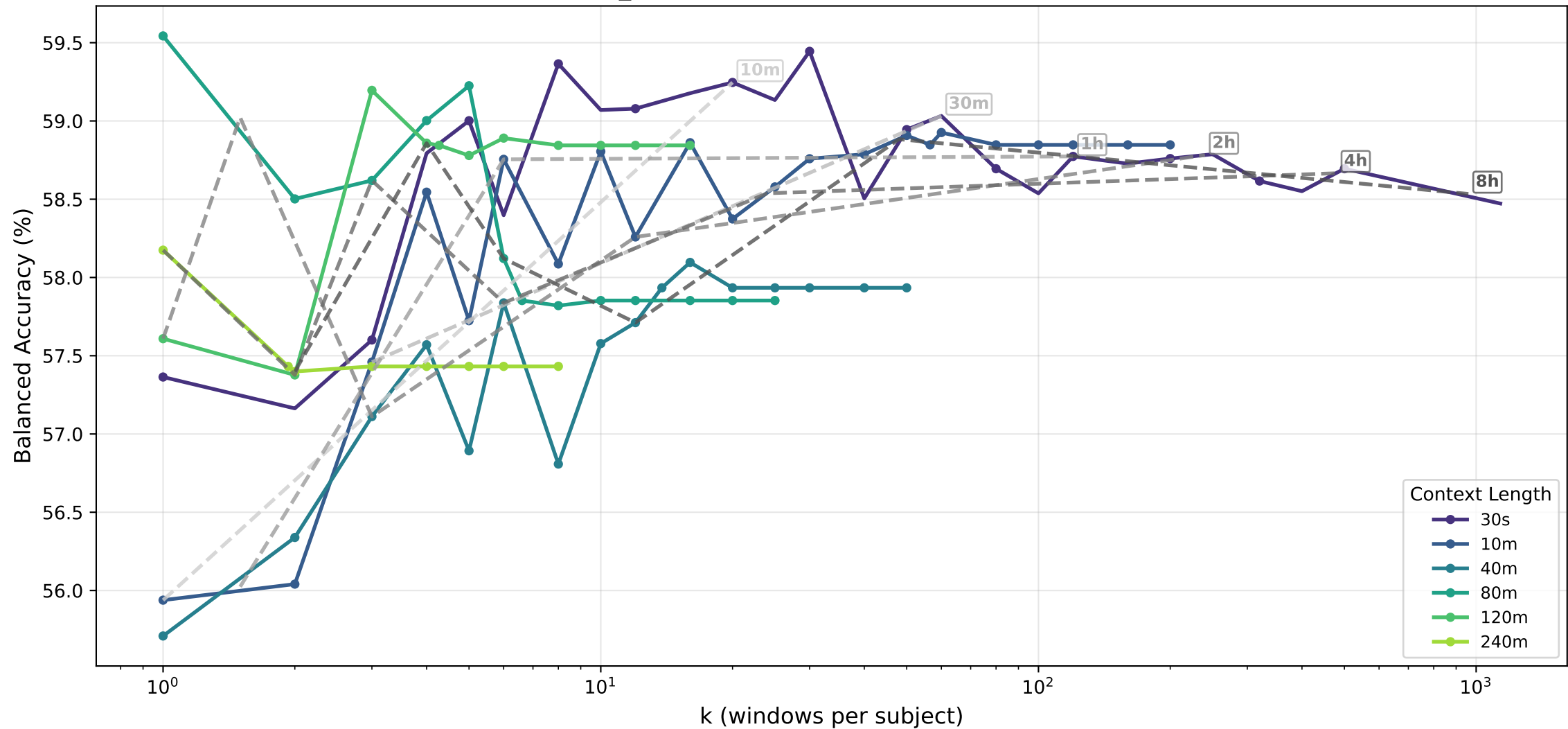
sleepiness_binary · lstm — Balanced Accuracy (%) vs k
