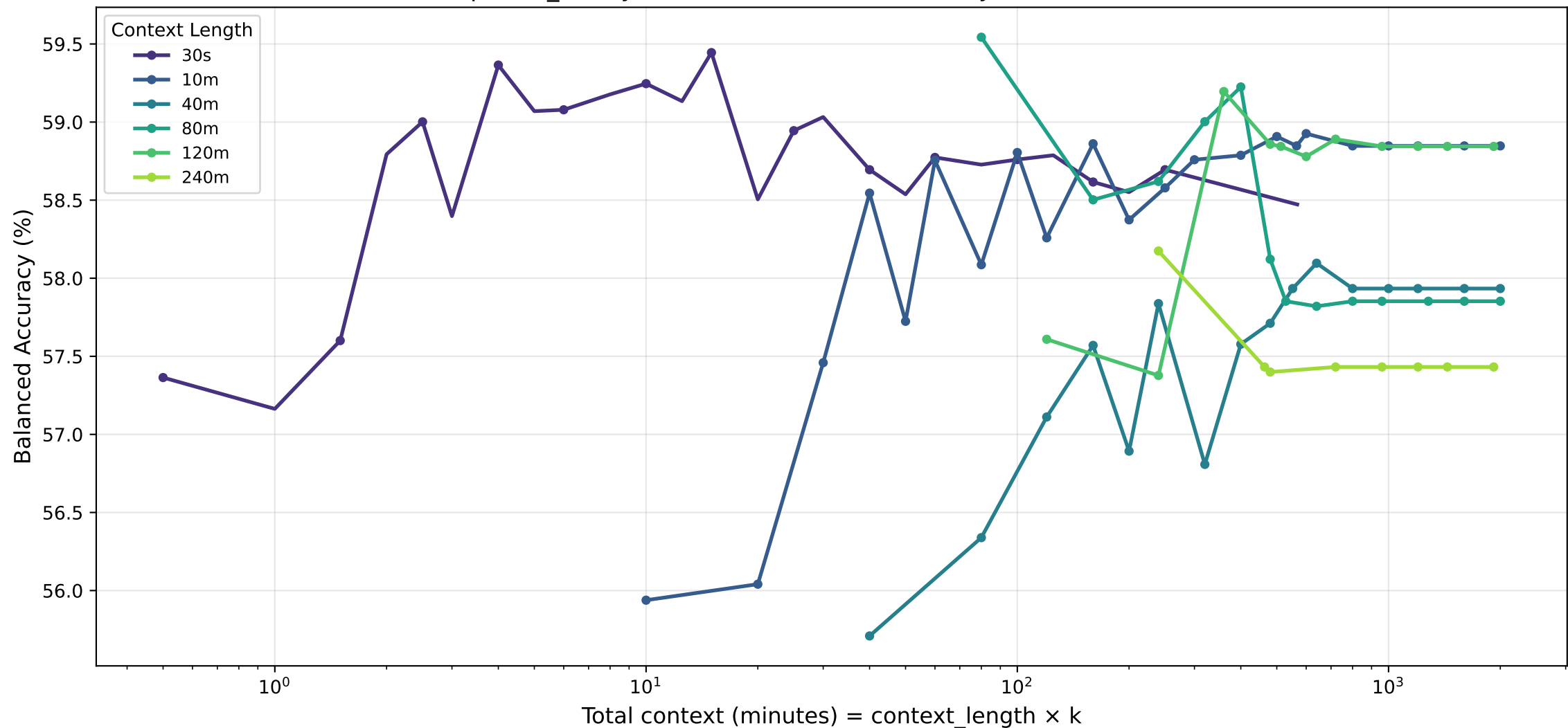
sleepiness_binary · Istm — Balanced Accuracy (%) vs Total Context
