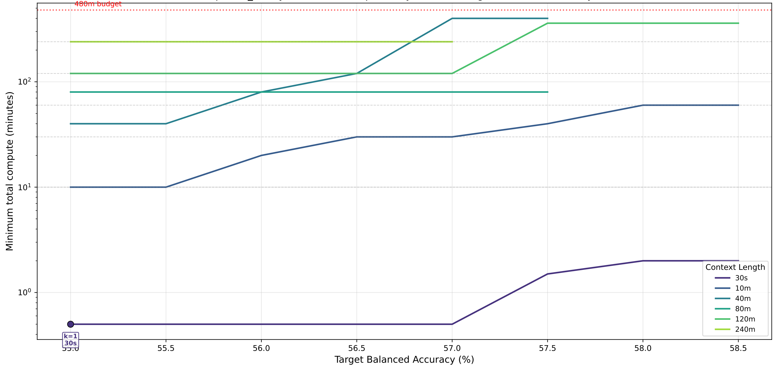
sleepiness_binary · Istm — Cheapest Way to Reach Target Balanced Accuracy (%)
