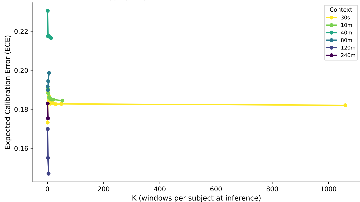
ECE vs K — sleepiness_binary (LSTM) Aggregating more windows reduces calibration error
