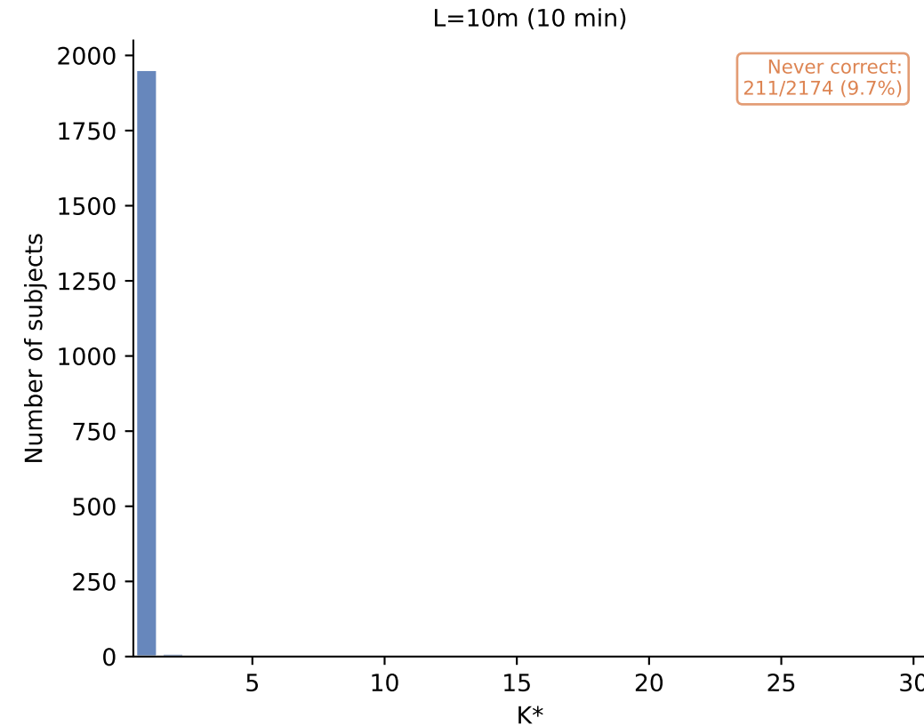
K* Distribution — sleepiness_binary (LSTM) K* = minimum windows for correct classification (reps=20)
