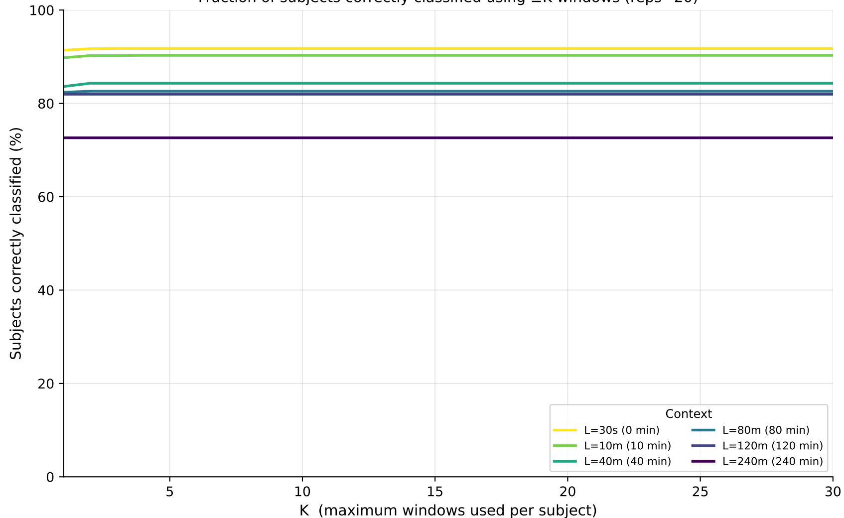
Coverage Curves — sleepiness_binary (LSTM) Fraction of subjects correctly classified using \leq K windows (reps=20)
