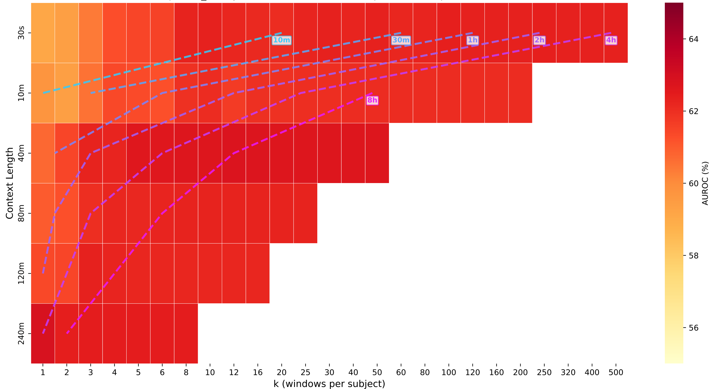
sleepiness_binary · transformer — Iso-Compute Heatmap: AUROC (%)
