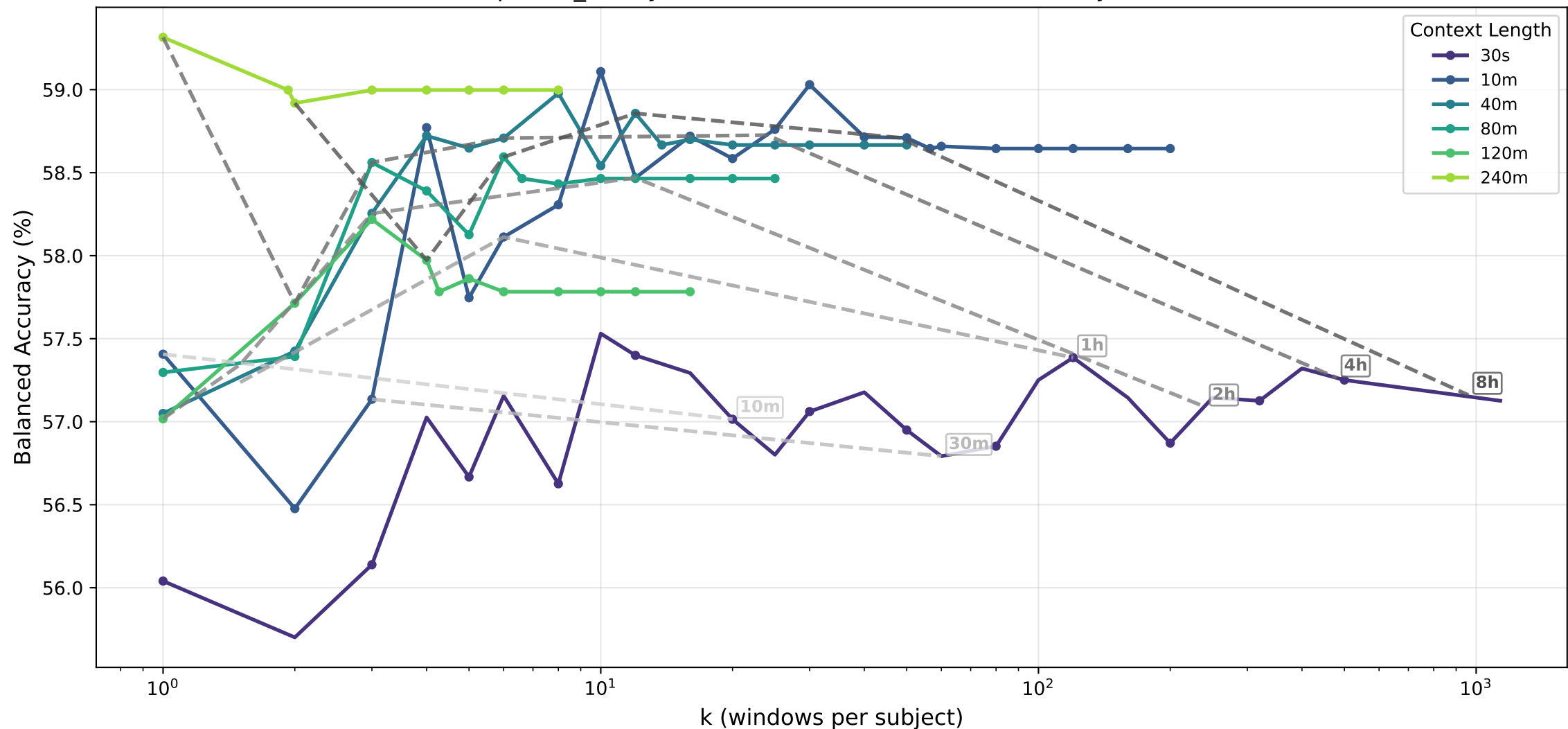
sleepiness_binary · transformer — Balanced Accuracy (%) vs k
