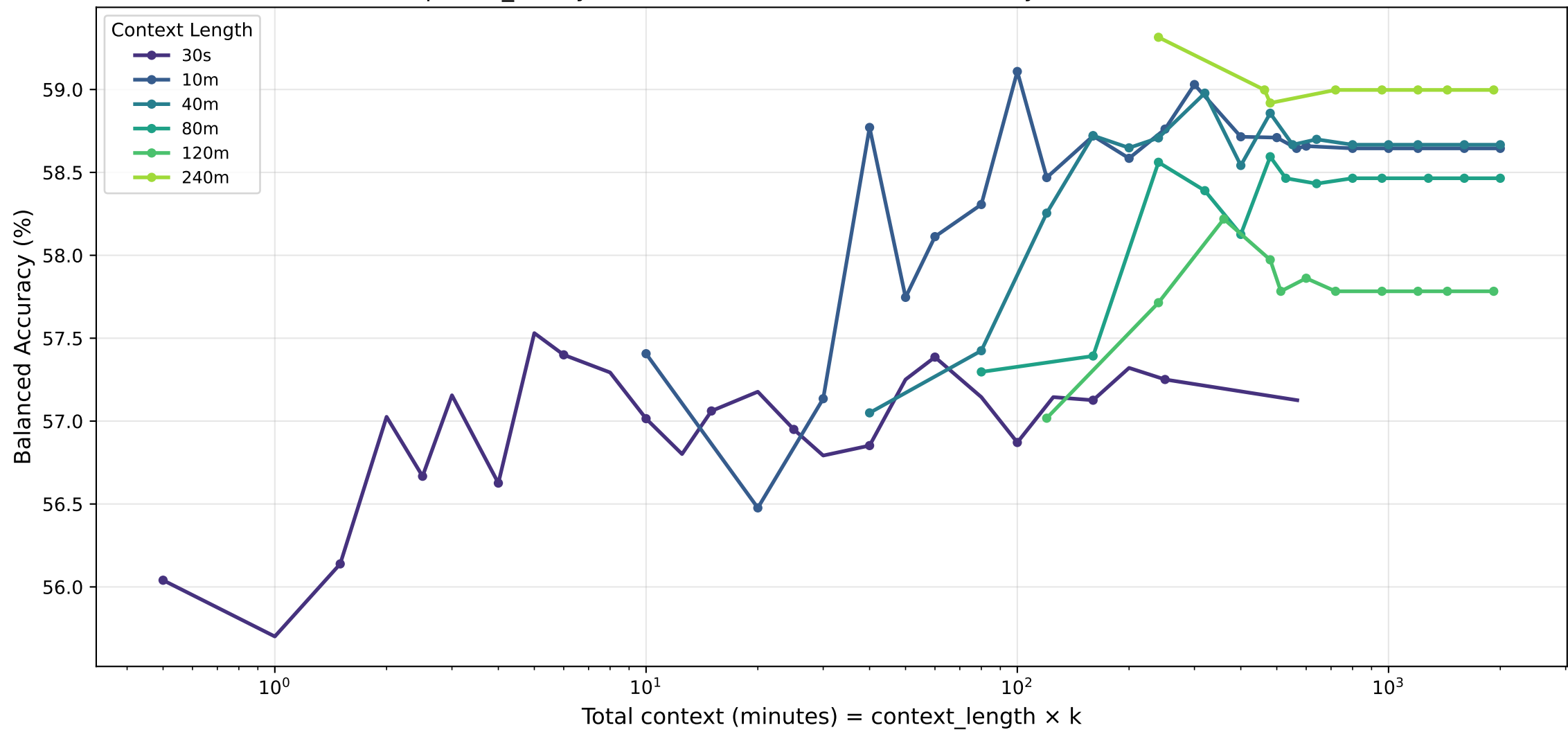
sleepiness_binary · transformer — Balanced Accuracy (%) vs Total Context
