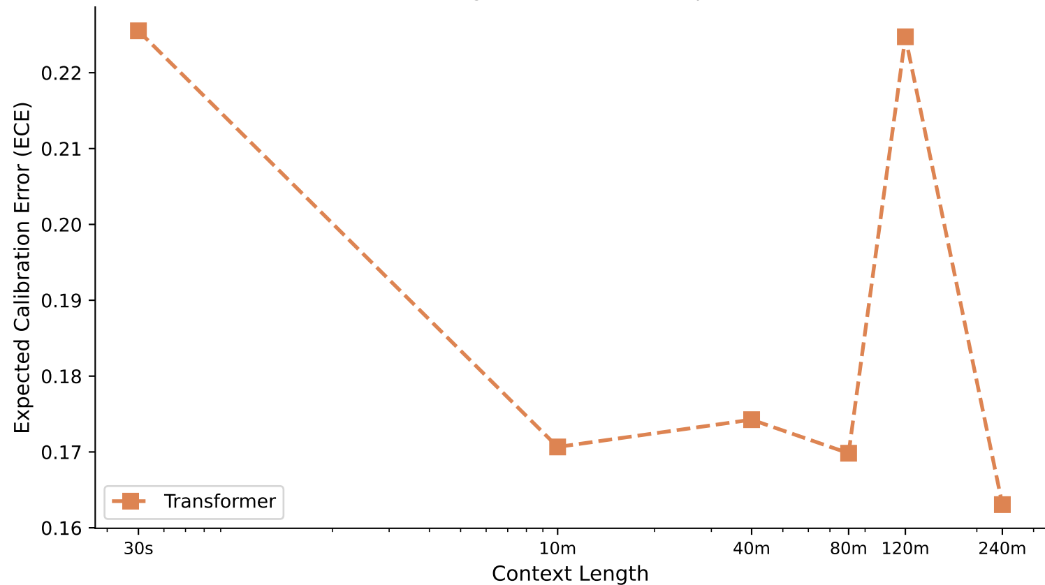
ECE vs Context Length — sleepiness_binary (K=10) Lower is better; longer context should improve calibration
