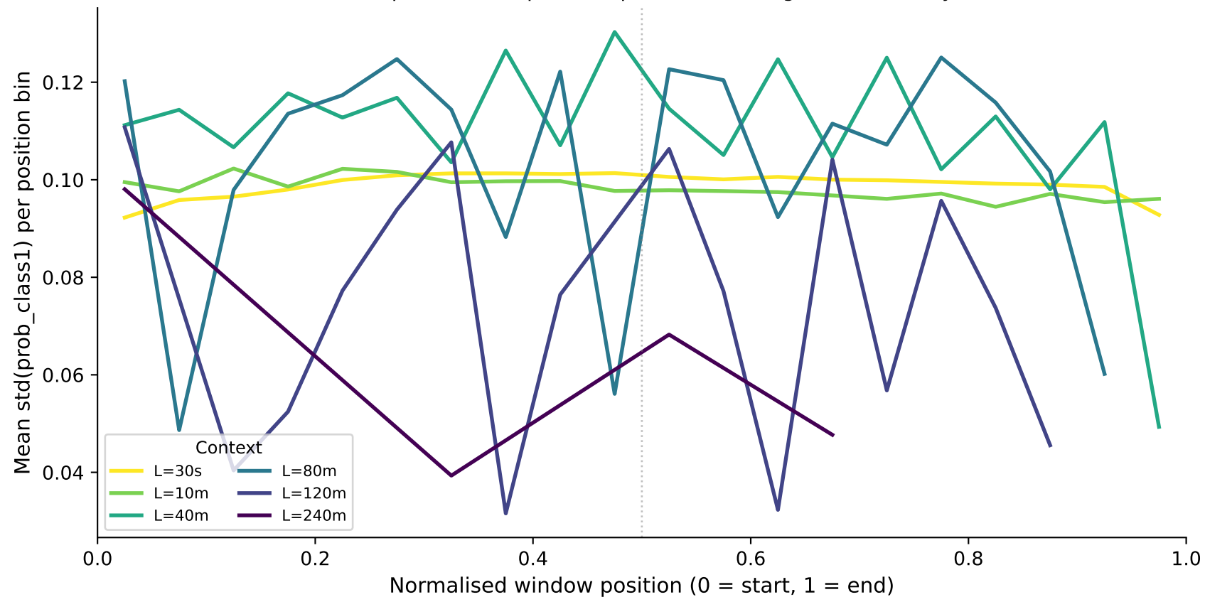
Prediction Variance vs Night Position — sleepiness_binary (TRANSFORMER) Lower variance = position-independent predictions (longer context may flatten this)
