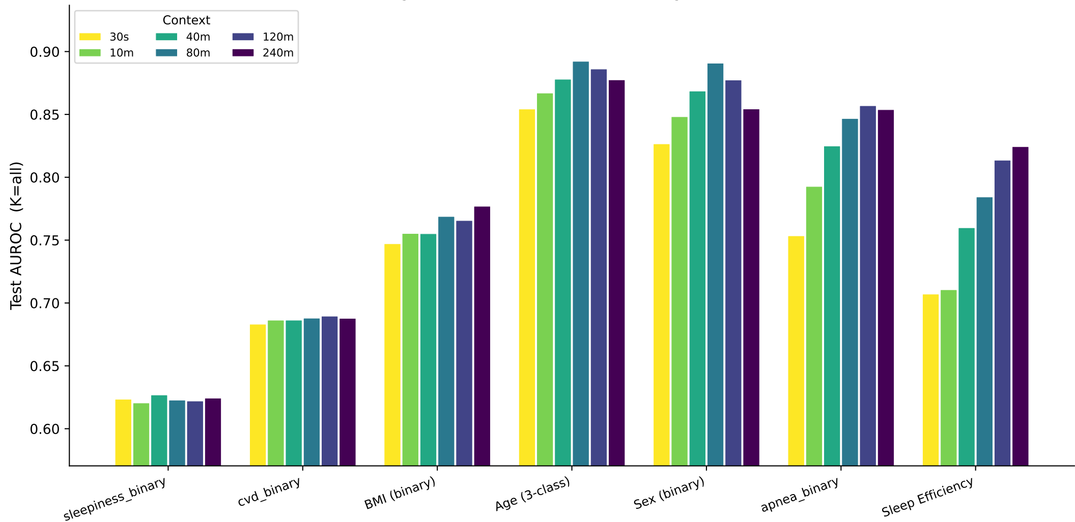
AUROC by Context Length per Task — TRANSFORMER (sorted by context sensitivity)
