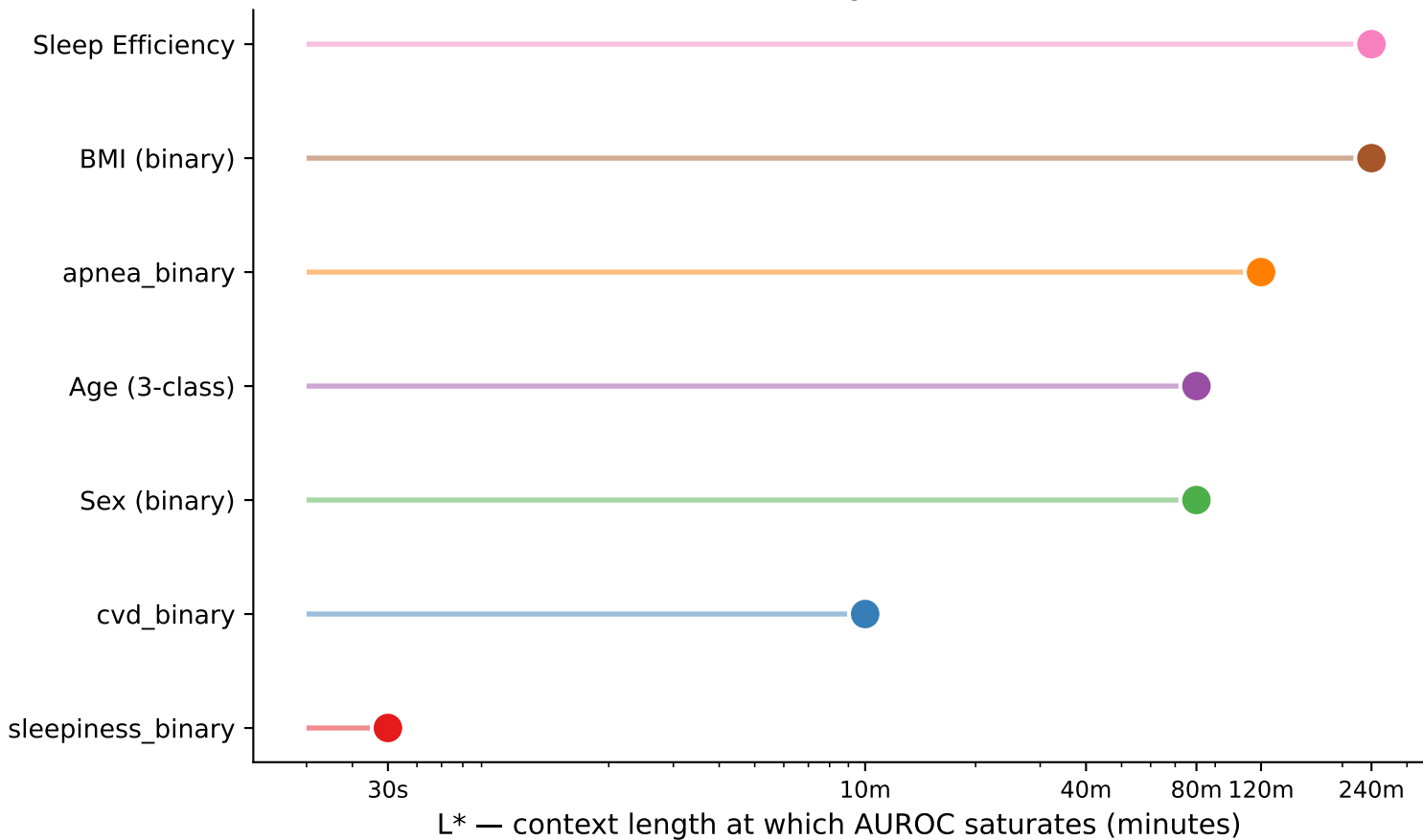
Task-Specific Saturation Context (L*) Minimum context to reach near-ceiling AUROC (within 0.5% of maximum)
