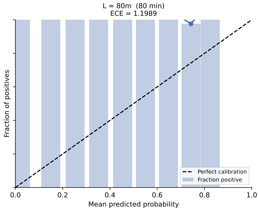
Reliability Diagrams — age_class (LSTM, K=10) Diagonal = perfect calibration
