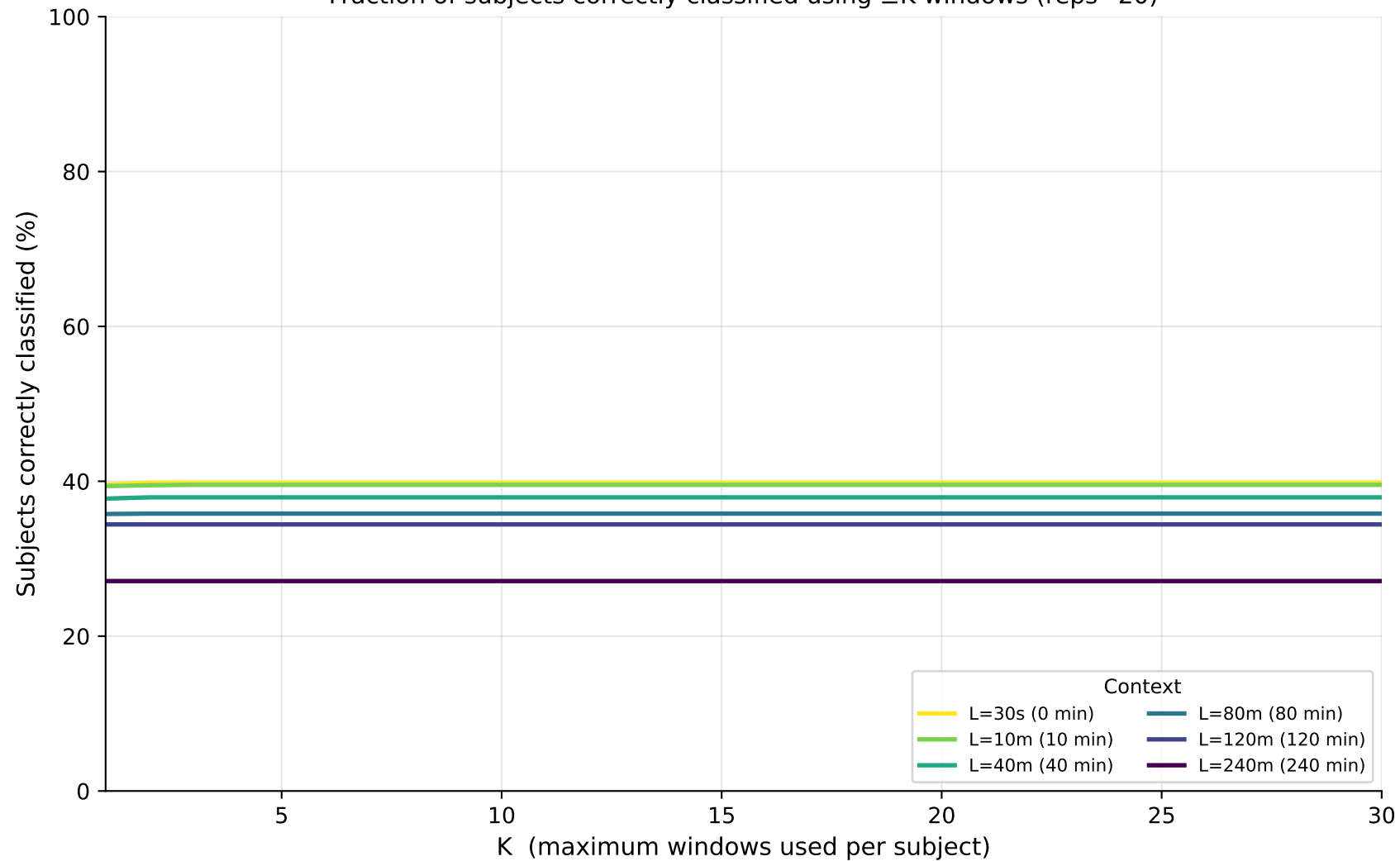
Coverage Curves — age_class (LSTM) Fraction of subjects correctly classified using \leq K windows (reps=20)
