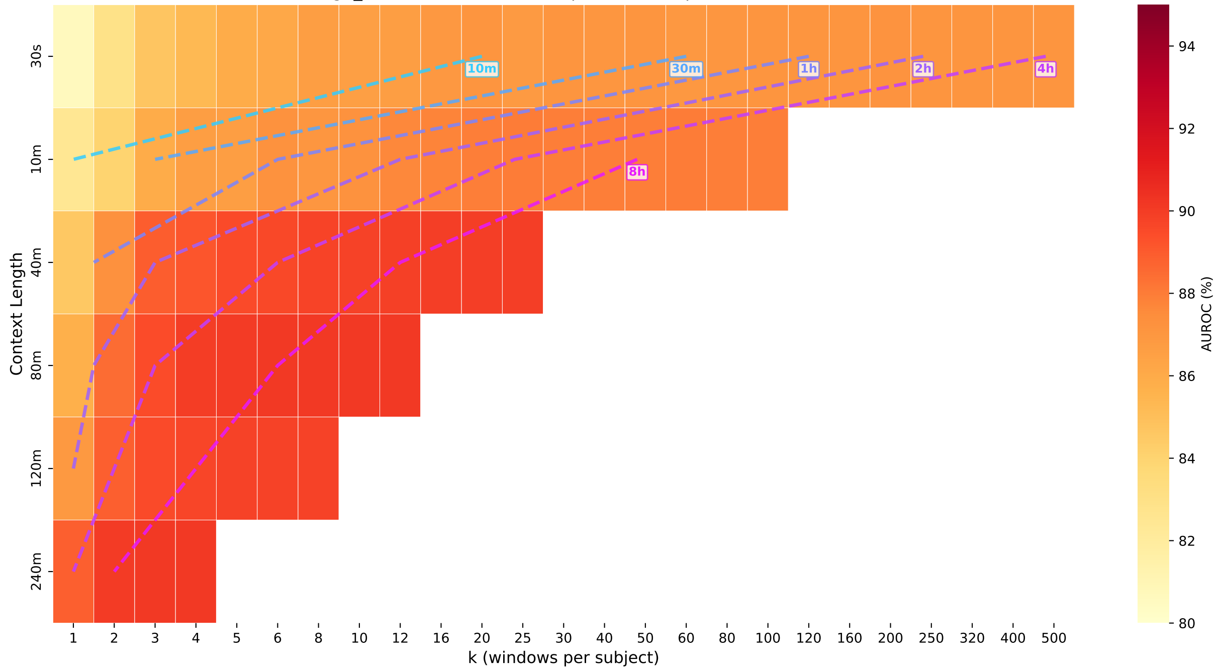
age_class · lstm — Iso-Compute Heatmap: AUROC (%)
