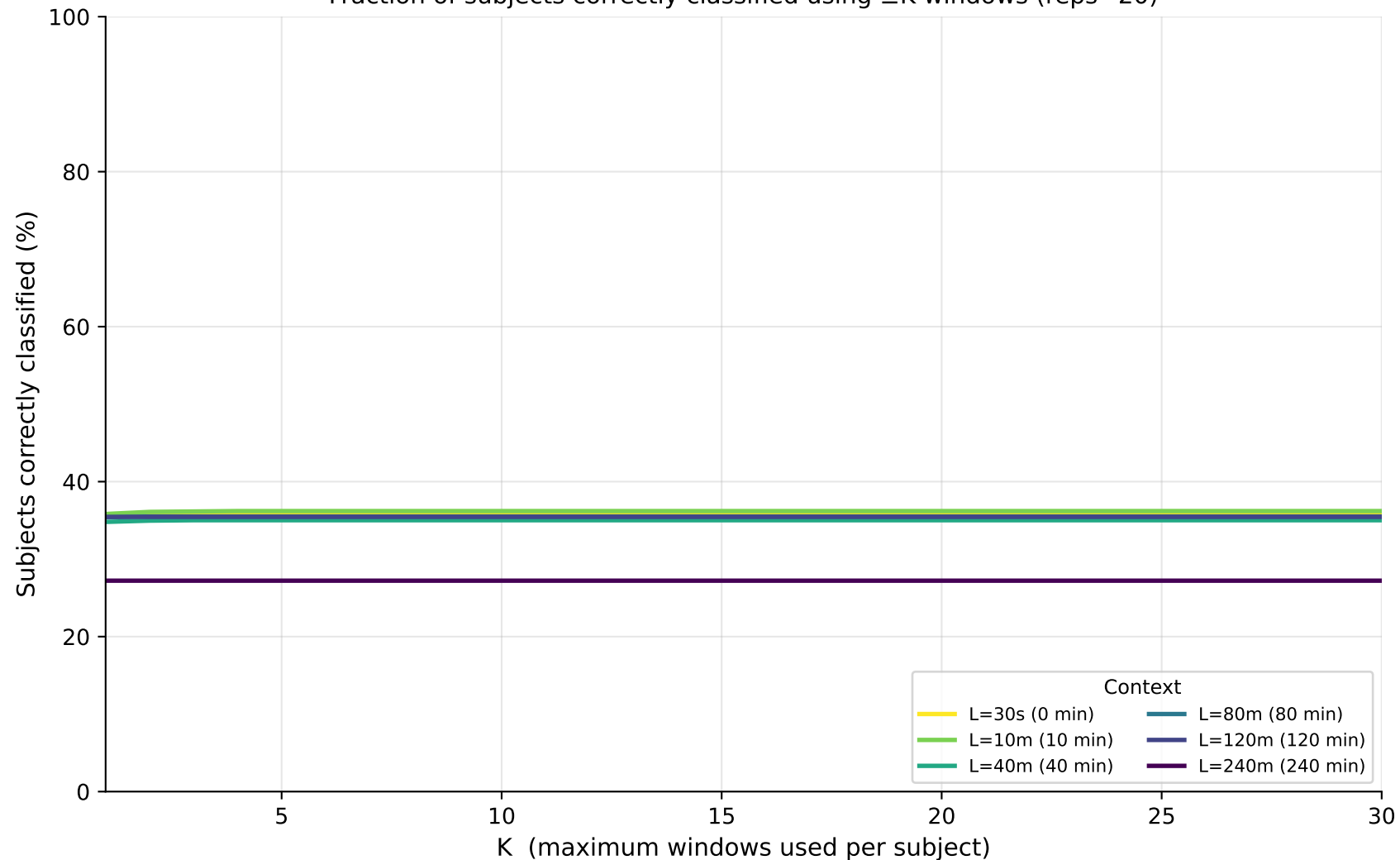
Coverage Curves — age_class (TRANSFORMER) Fraction of subjects correctly classified using \leq K windows (reps=20)
