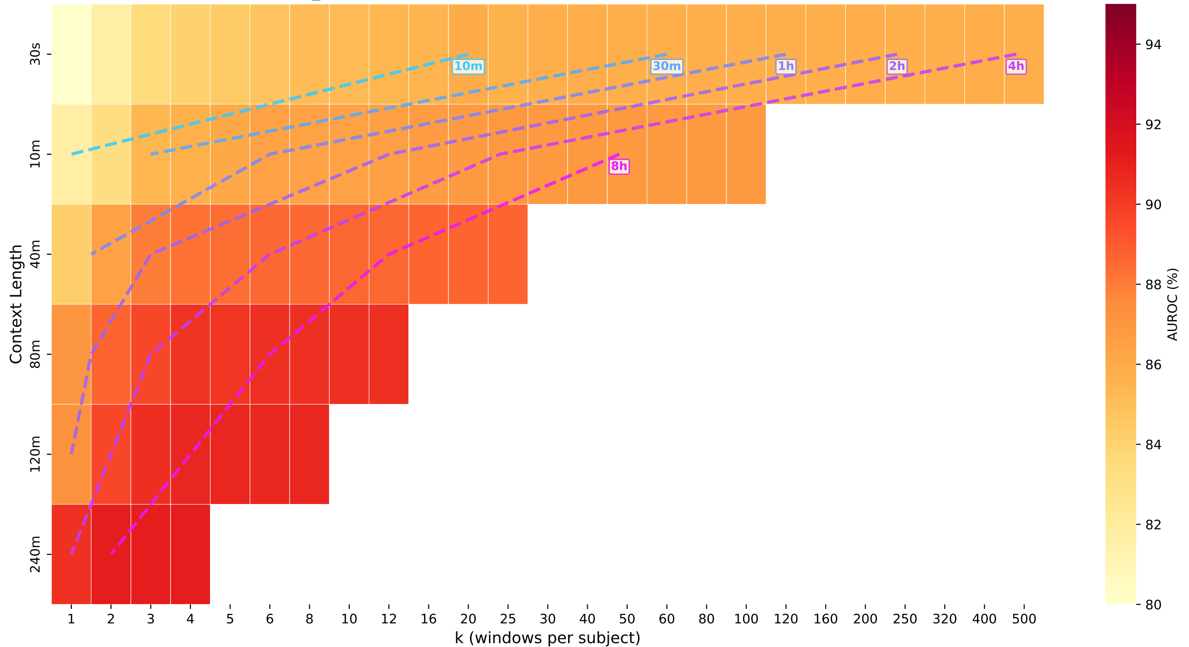
age_class · transformer — Iso-Compute Heatmap: AUROC (%)
