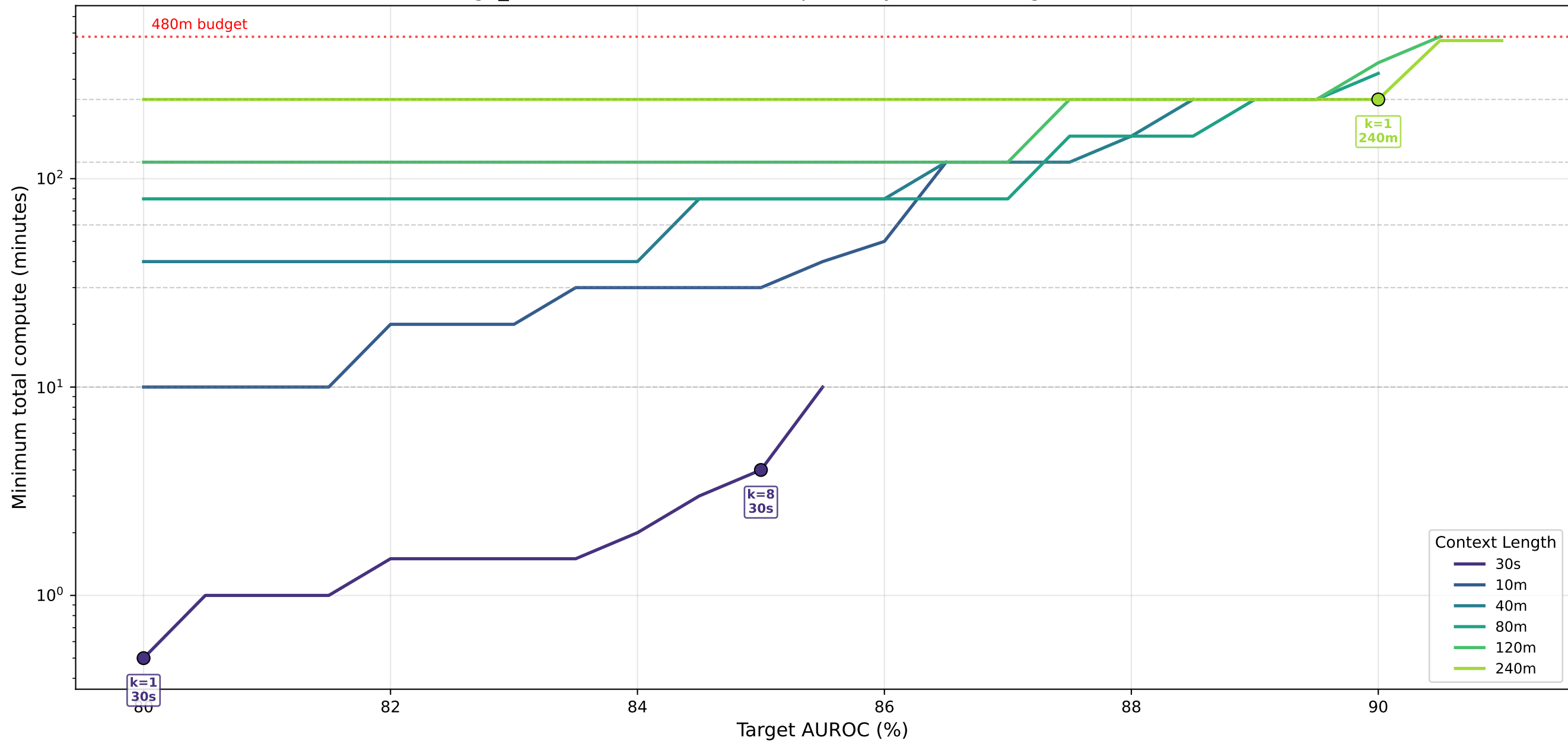
age_class · transformer — Cheapest Way to Reach Target AUROC (%)
