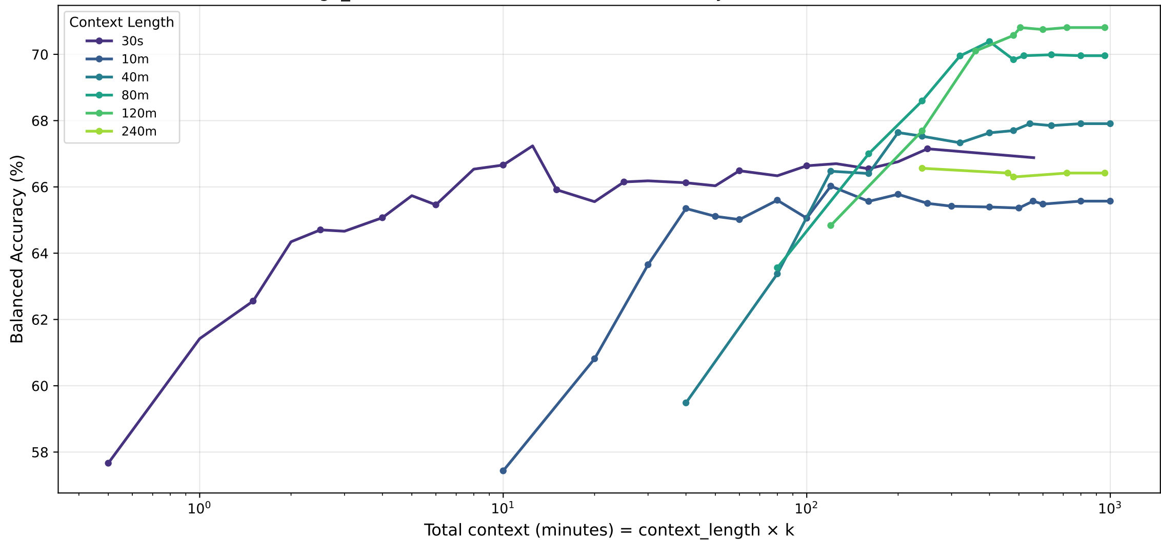
age_class · transformer — Balanced Accuracy (%) vs Total Context
