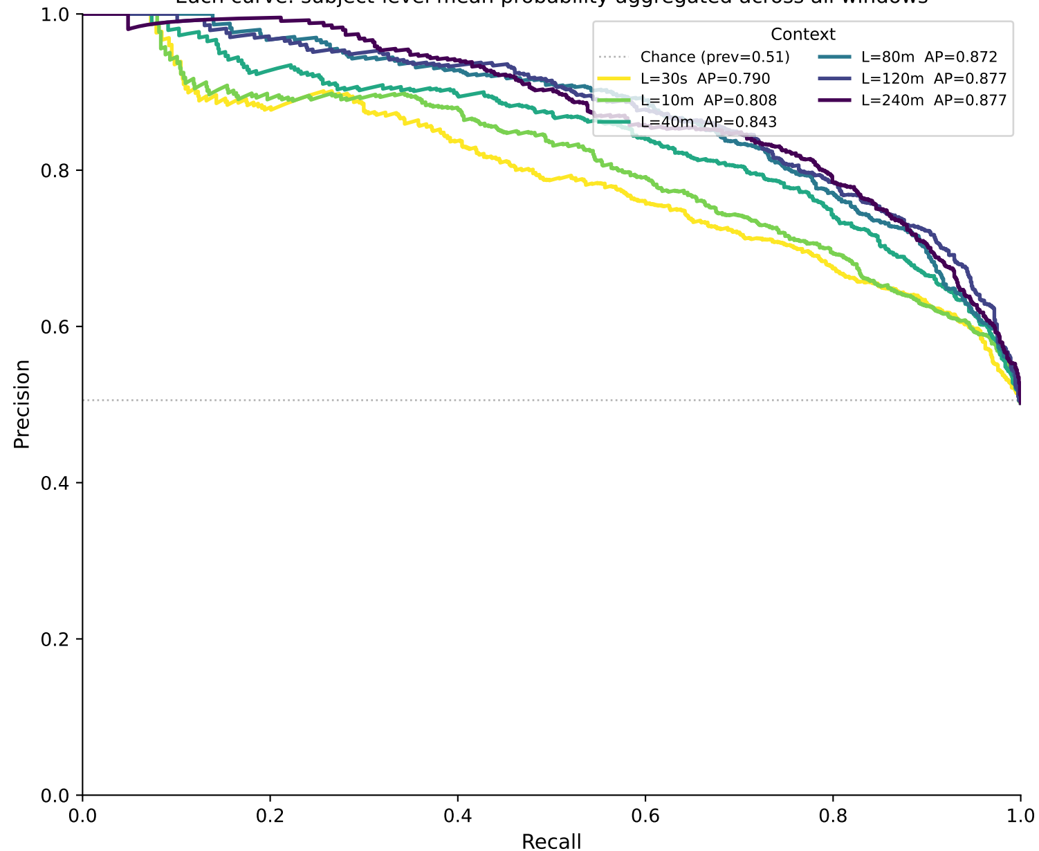
Precision-Recall Curves — apnea_binary (LSTM) K=all Each curve: subject-level mean probability aggregated across all windows
